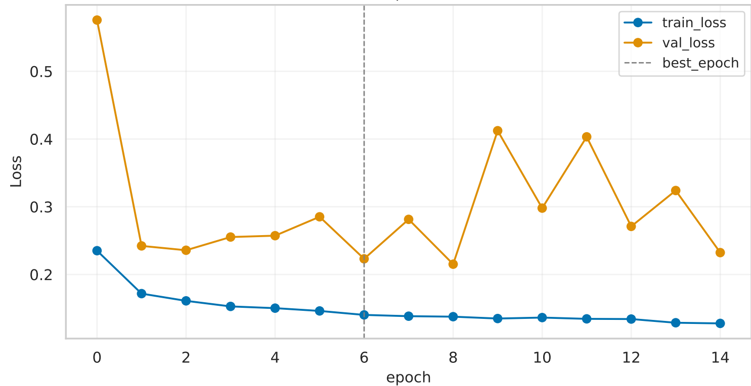
resnet34 | Loss curves
