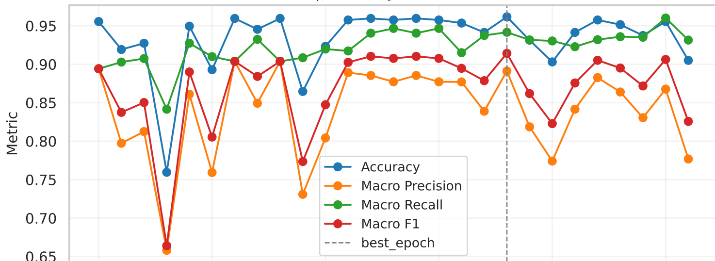
resnet34 | Accuracy/Precision/Recall/F1
