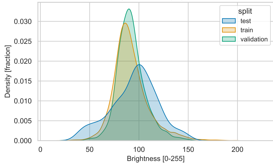
Brightness density by split
