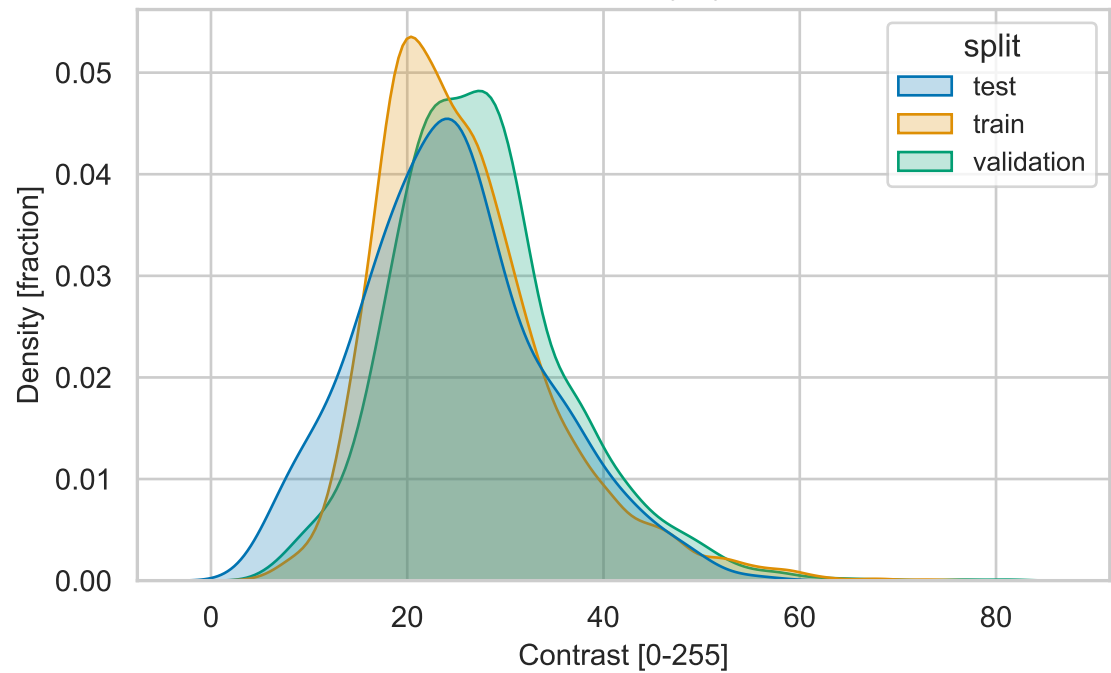
Contrast density by split
