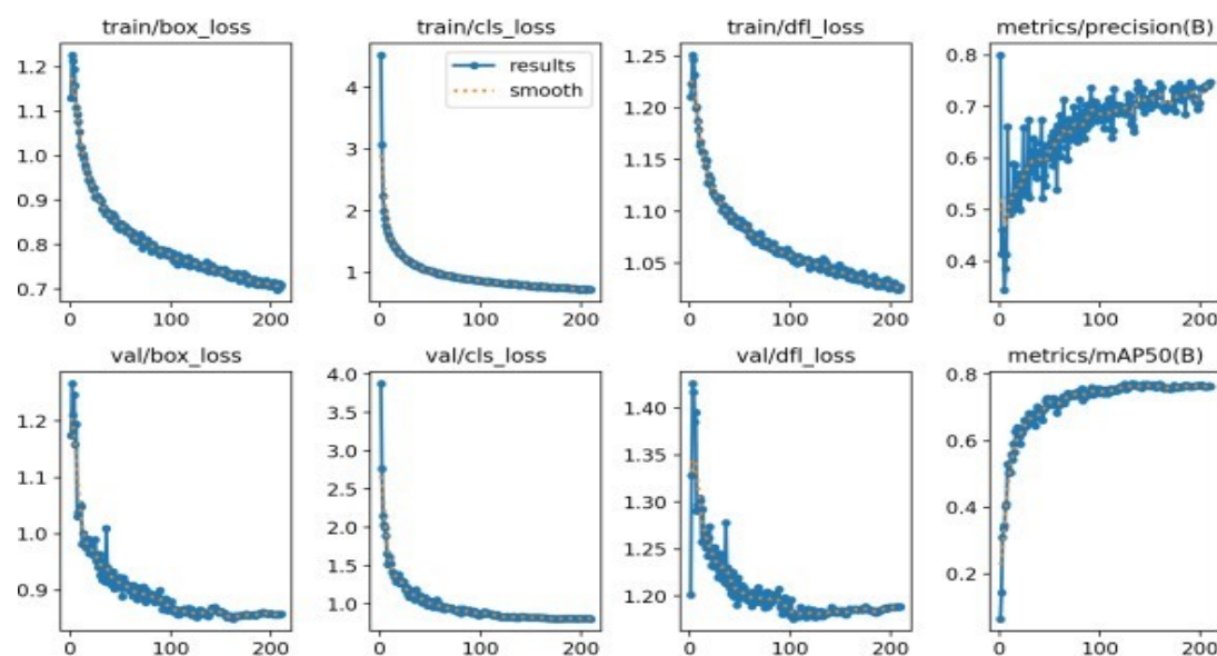
Figure 4 Performance Metrics
