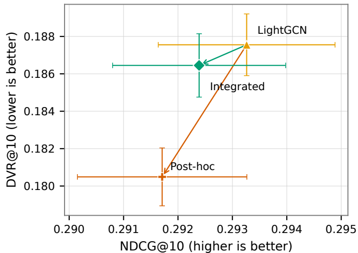
(b) Matched LightGCN operating points
