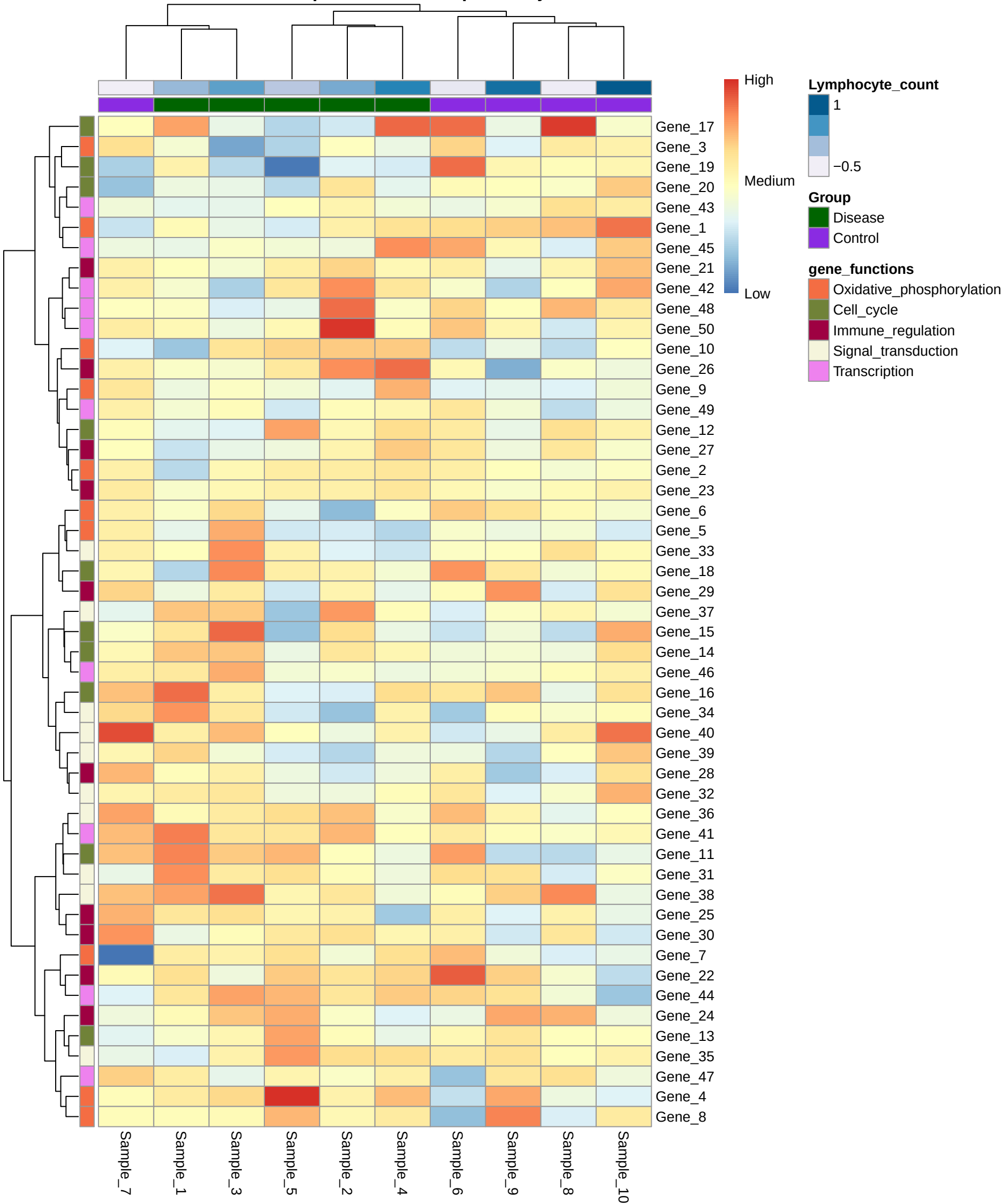
Annotated Gene Expression Heatmap for Project test
