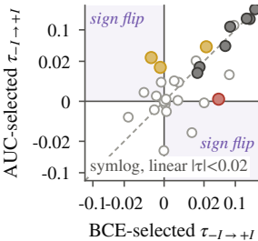
(a) Selector only ( -\Delta_{DP} )
