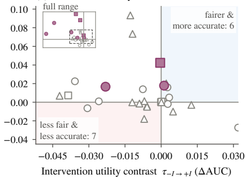
(b) Intervention utility–fairness trade-off
