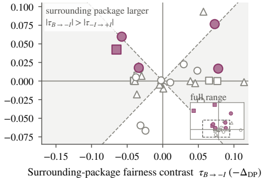
(a) Fairness attribution
