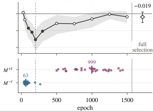
(b) FairGB / Bail ( H = 1500 )
