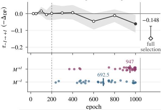
(a) NIFTY / German (published drop rates, H = 1000 )
