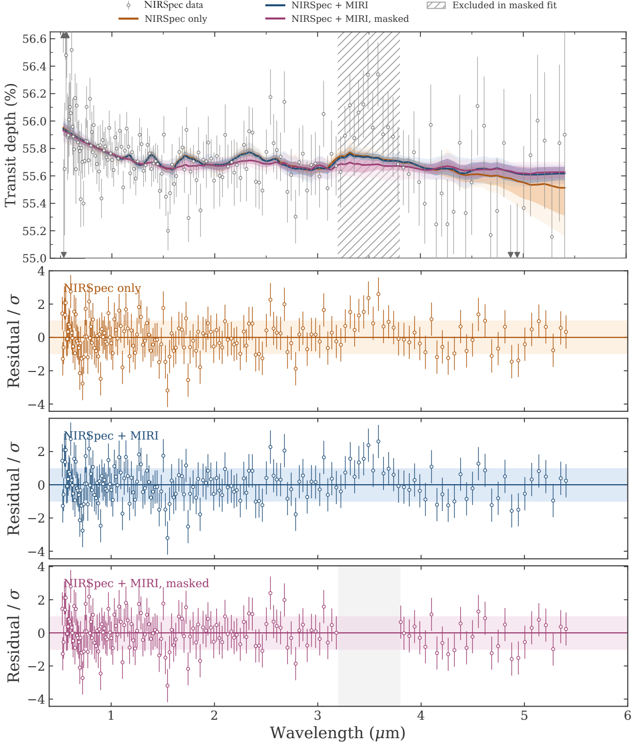
Figure 5. Measured NIRSpect data binned to a resolution of R_{\text{bin}} = 75 prior to conducting the retrieval (see text for details). We present retrieved spectra from three different runs: NIRSpect only (orange), NIRSpect+MIRI (blue), and NIRSpect+MIRI excluding the 3.2–3.8 \mu\text{m} data (purple). We suspect that an unknown hydrocarbon feature in this spectral region, denoted by the hash marks, is artificially biasing the methane abundance to higher values. When we remove these wavelengths, the prominent methane bumps are no longer required by the data. We additionally find that the long-wavelength tail ( \geq 4 \mu\text{m} ) is much more strongly constrained when the MIRI observations are included in the retrievals.
