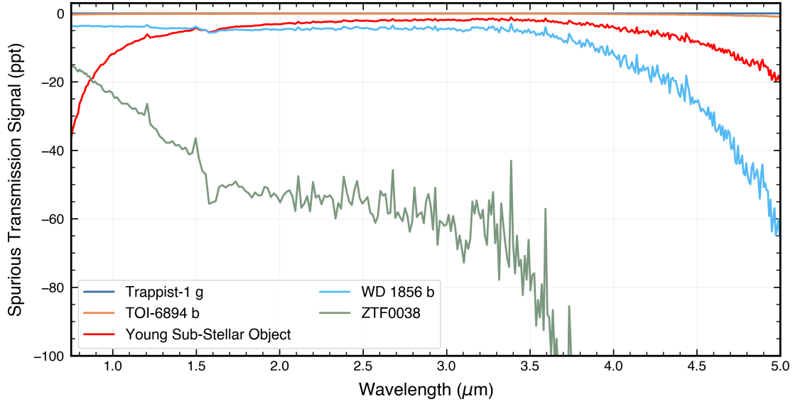
Figure 11. Spurious signal produced by background contamination \Delta d_\lambda for several systems: Trappist-1 g, a giant planet around a 0.2 M_\odot star (TOI-6894 b), an eclipsing white dwarf (ZTFJ0038+2030, referred to as ZTFJ0038 in the figure), and a theoretical young, sub-stellar object with a transiting companion. We find that this contamination is most relevant for faint systems, such as white dwarfs and sub-stellar objects. We note that this assumes no background correction, and therefore provides an upper bound on the spurious signal.
