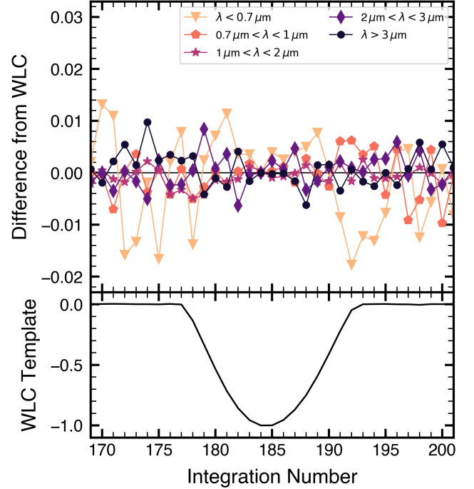
Figure 4. Chromatic limb darkening check. We compare the difference between the empirical light curves in different wavelength bins relative to the white light curve (WLC). We find that chromatic limb darkening will have a negligible effect for wavelengths > 0.7 \mu\text{m} , but may cause us to underestimate the transit depths at PRISM's bluest wavelengths.
