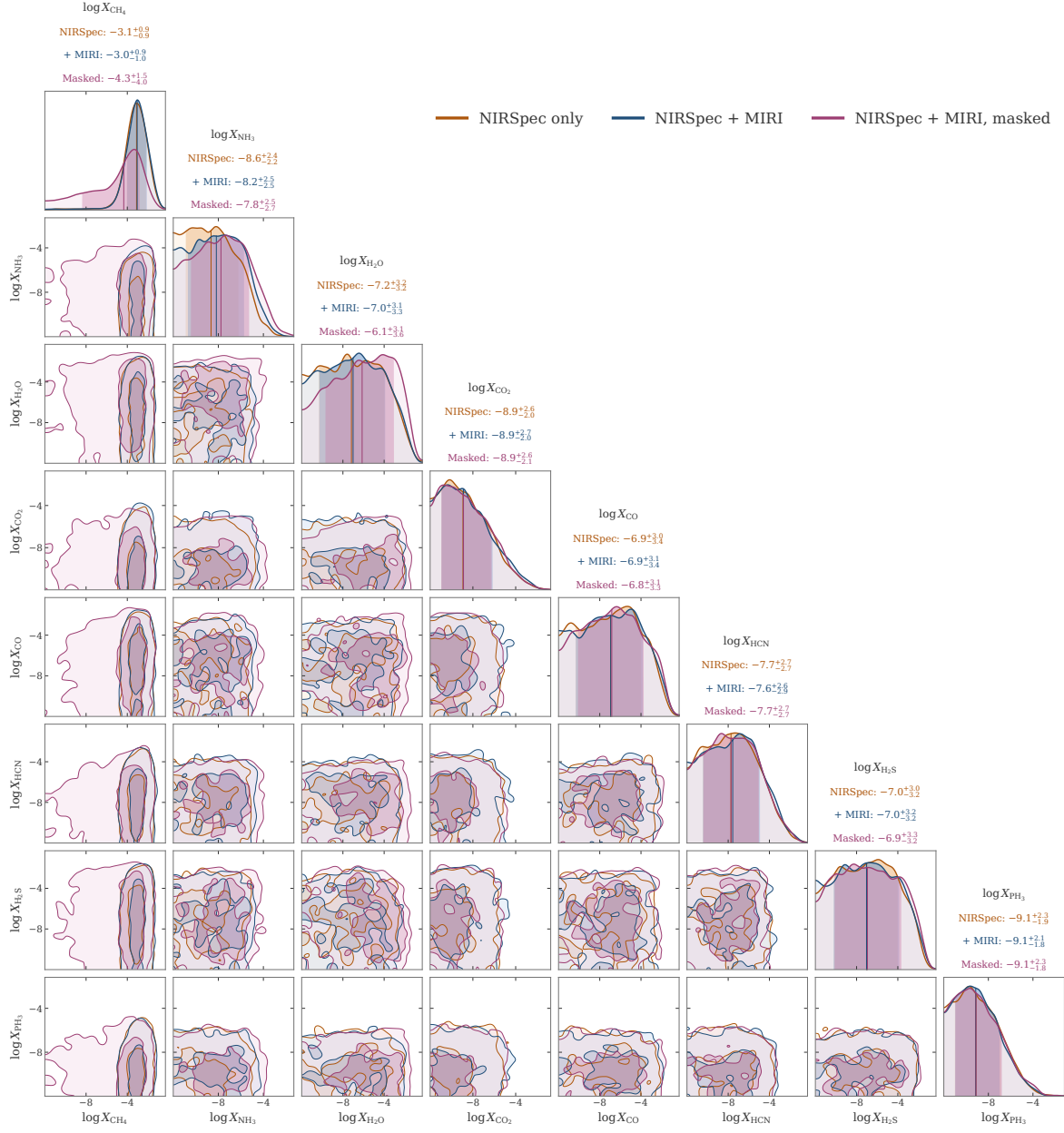
Figure 12. Other than methane, no other species included in our retrieval are detected. The corner plot shows a stable abundance for methane in the NIRSpec-only, NIRSpec+MIRI, and masked NIRSpec+MIRI retrievals, although we find that this becomes only an upper limit when the 3.2-3.8 \mu\text{m} data is excluded from the retrieval.
