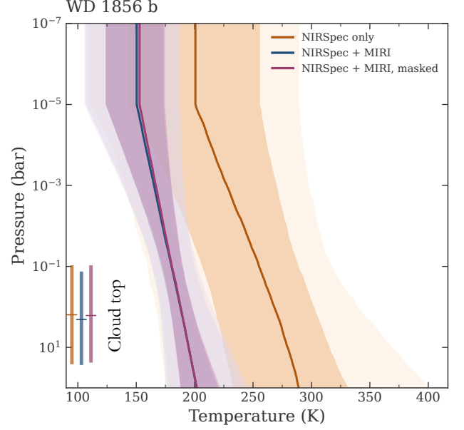
Figure 7. We use a simple 2-node temperature prior for our retrievals.
