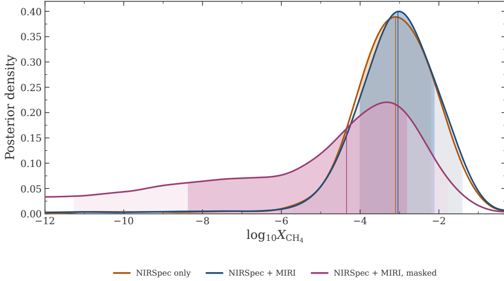
Figure 8. Methane abundance for the three different retrieval runs. If the 3.2\text{--}3.8\ \mu\text{m} data is included, the retrieved methane abundance is \log_{10} X_{\text{CH}_4} \approx -3 and well constrained. However, if the 3.2\text{--}3.8\ \mu\text{m} data is removed, we find the methane abundance becomes an upper limit, suggesting that the detection was driven by the unknown, Saturn-like hydrocarbon feature. Methane is certainly still allowed at \log_{10} X_{\text{CH}_4} < -3 ( 1\sigma upper bound), but will require additional transits to confirm the opacity and determine the abundance.
