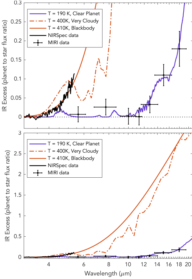
Figure 1. PLACEHOLDER Top : NIRSpec/PRISM and MIRI imaging observations. NIRSpec data is consistent with a \sim 400 K planet, demonstrated by the blackbody and cloudy models (red curves), while MIRI data is consistent with a much colder \sim 190 K planet (blue curve). Bottom : Zoomed-out comparison. The best-fit NIRSpec temperature is highly discrepant with the MIRI observations.
