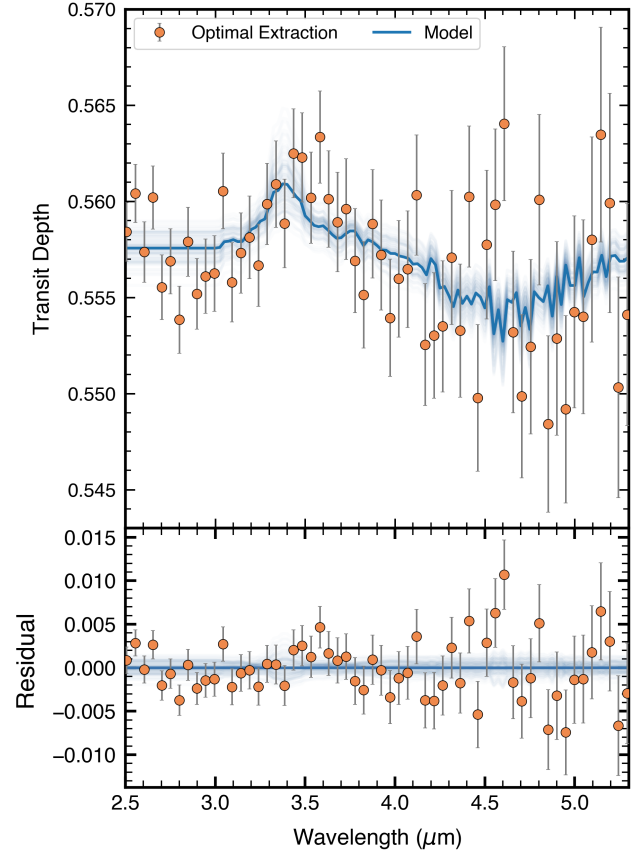
Figure 10. Best-fit model for the unidentified spectral feature at \sim 3.4 \mu\text{m} , calculated using scaled observations of a corresponding feature in Saturn’s spectrum. We use this to perform a secondary measurement of the planet’s mass (see §5).
