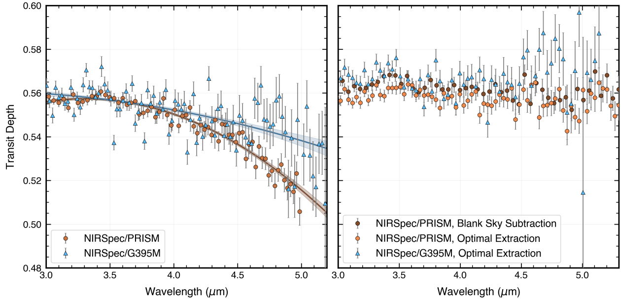
Figure 2. Left: Comparison between NIRSpec/PRISM and NIRSpec/G395M data, denoted by orange circles and blue triangles, respectively. To guide the eye, we also show best-fit quadratic fits to both datasets within the 3–5.2 \mu\text{m} region, with corresponding 1\sigma uncertainties denoted by the shaded regions. Right: Corrected NIRSpec/PRISM observations. We subtract the background emission using a blank-sky observation (light orange) and an optimal extraction pipeline (dark orange). We find that both methods largely eliminate the apparent thermal slope.
