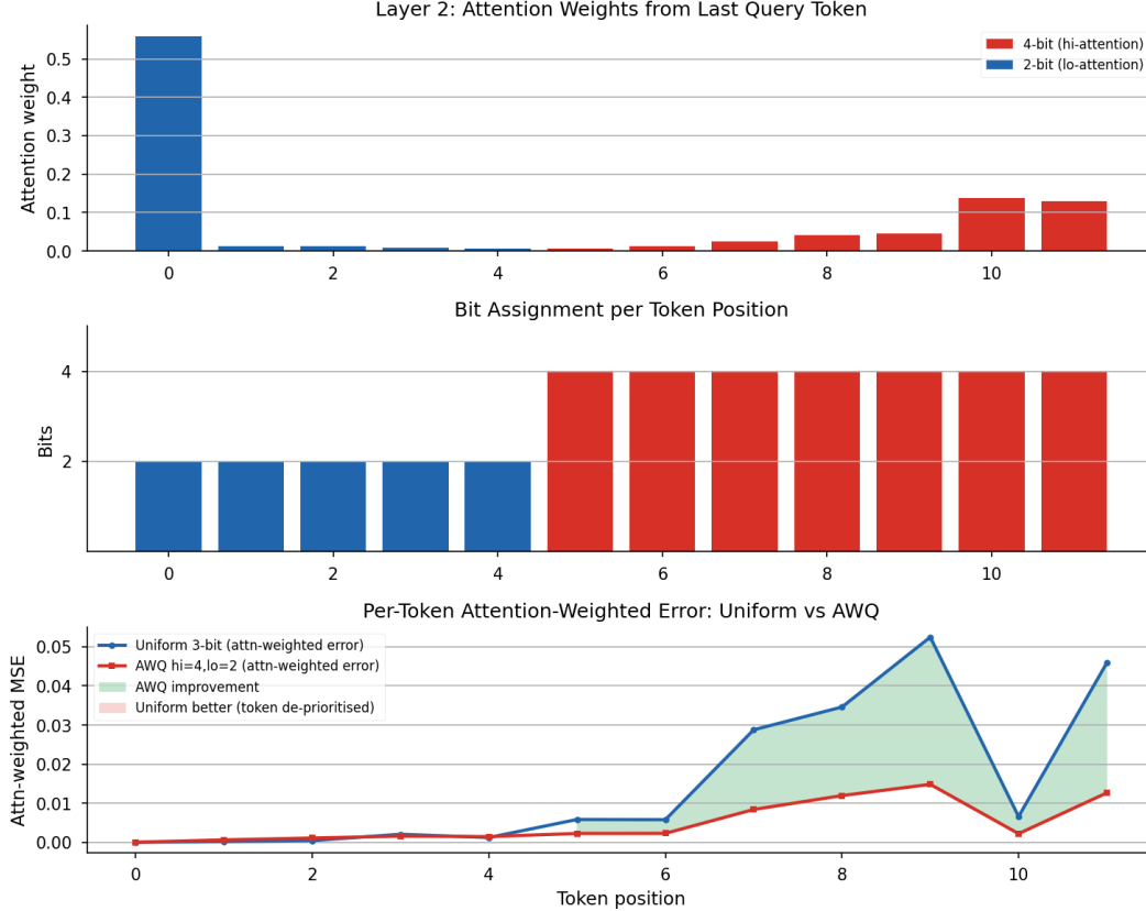
Figure 4: Attention-weighted quantization on distilgpt2 layer 2. Top: attention weights from the last query token, coloured by assigned bit-width. Middle: bit assignment per position. Bottom: per-token attention-weighted error for uniform 3-bit vs. AWQ (hi=4, lo=2).
