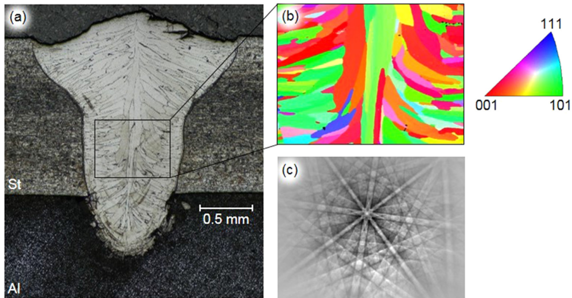
Fig. 22. EBSD of St-Al weld with penetration depths of \sim 500 \mu\text{m} . SEM of St/Al weld (a), inverse pole figure color map (b), Kikuchi diffraction pattern (c).
