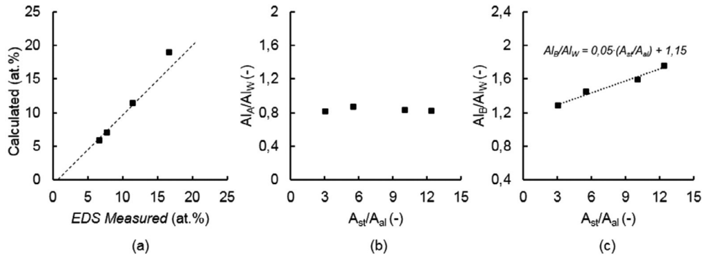
Fig. 10. Calculated versus measured average Al concentration in the St-Al welds (a). Correlation of the average aluminum concentration in the whole St-Al weld to the average aluminum concentrations in zone A (b) and zone B (c).
