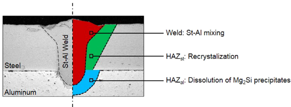
Fig. 3. Microstructural evolution in the St-Al joint.
