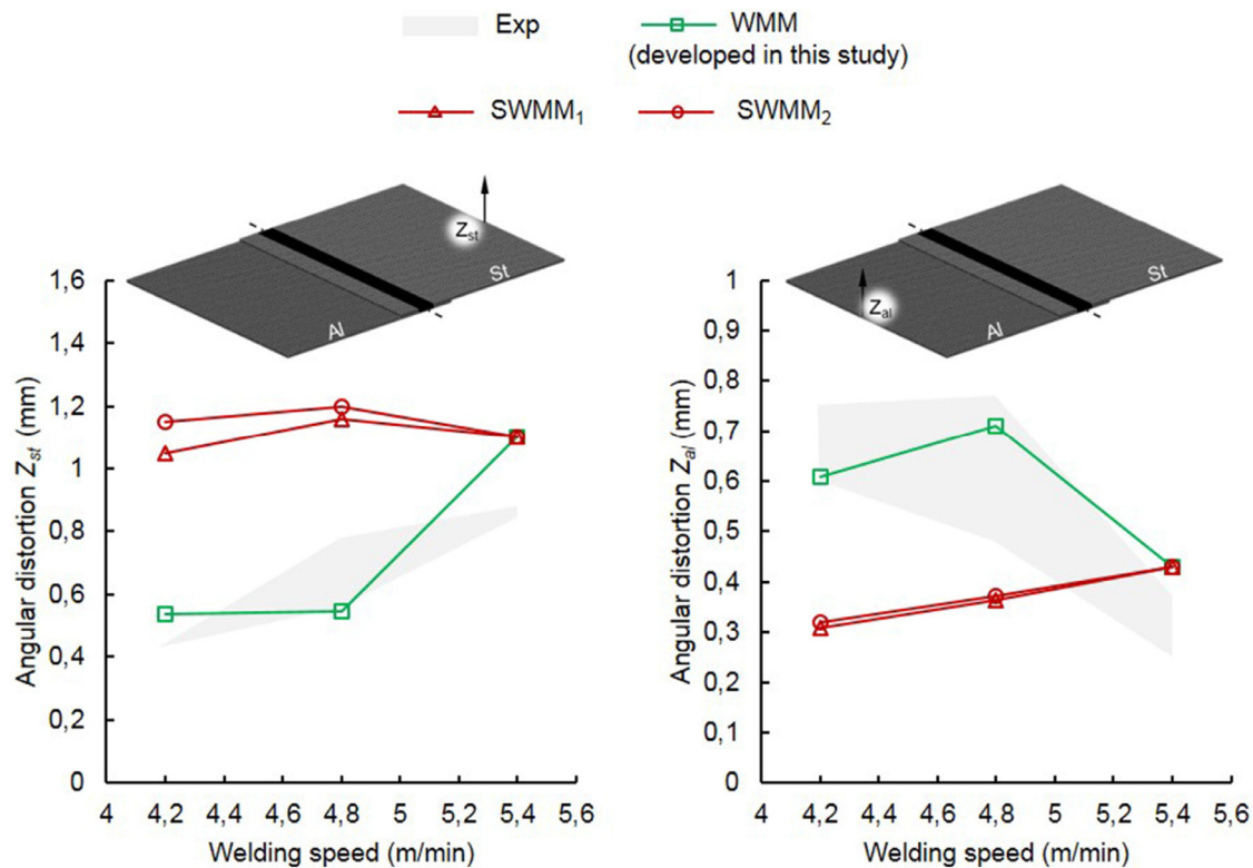
Fig. 24. Variation in prediction accuracy, when computing angular distortions using different weld material models. SWMM 1 approximates the elastic-plastic behavior of the St-Al weld metal by the mechanical properties of the steel, SWMM 2 uses the linear mixture rule to calculate the resulting mechanical properties and WMM is a developed weld material model as described in Section 3.2. P_L = 3.75 kW.
