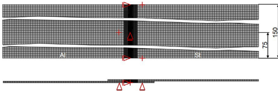
Fig. 14. Scheme of mechanical constraints after welding (unclamped condition).
