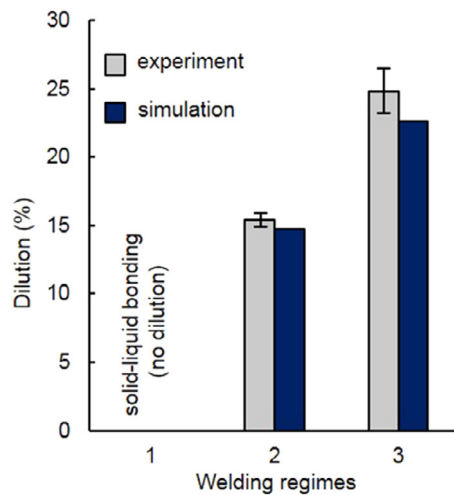
Fig. 17. Computed versus measured dilutions.
