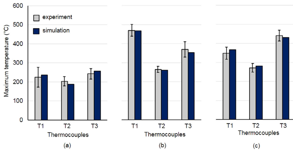
Fig. 16. Computed versus measured maximum temperatures. P_L = 3.75 kW.
