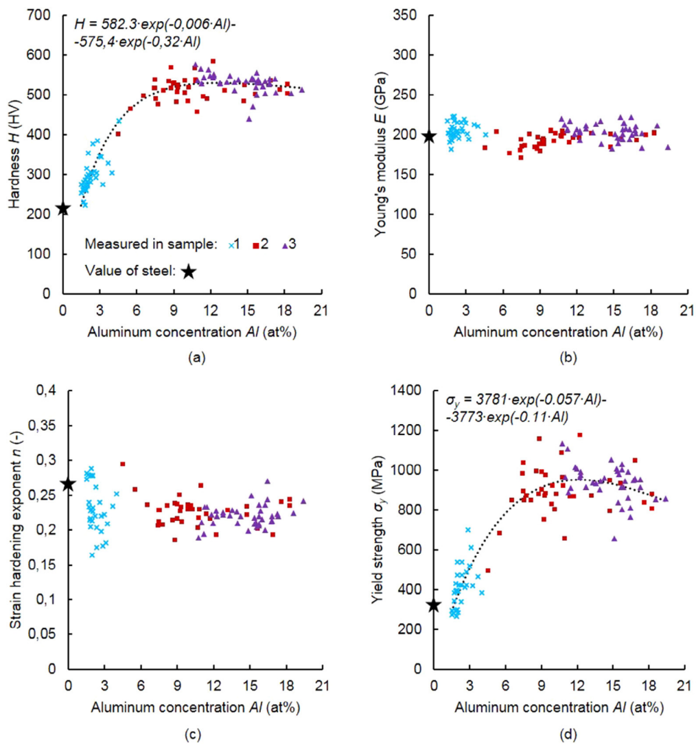
Fig. 8. Hardness (a), Young's modulus (b), strain hardening exponent (c) and yield strength (d) of the St-Al weld metal as a function of the aluminum concentration. Samples 1-3 according to Fig. 7.
