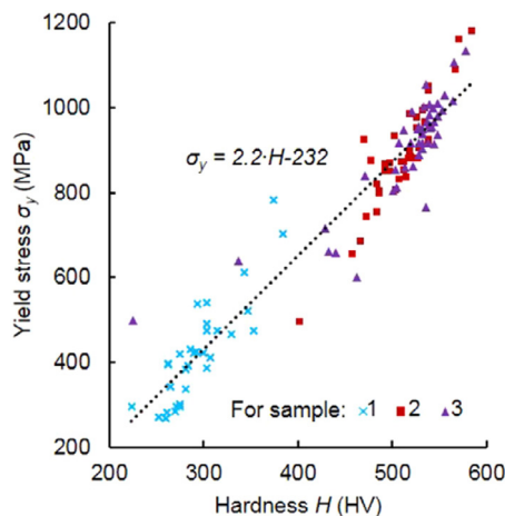
Fig. 23. Yield strength vs. hardness of St-Al weld metal. Samples 1-3 according to Fig. 7.
