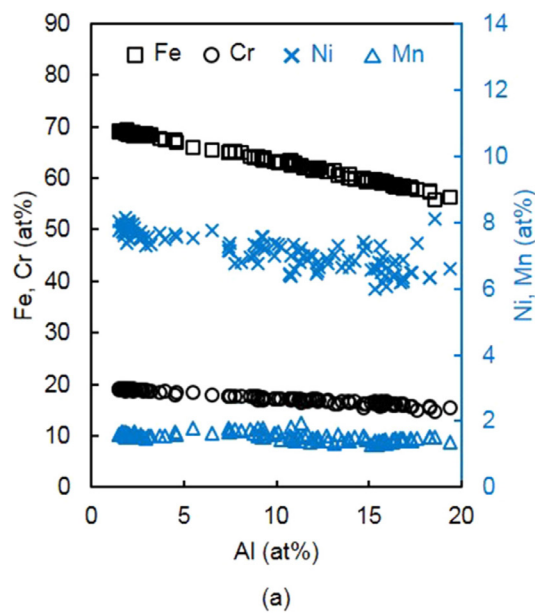
Fig. 21. Measured chemical composition (a) and calculated corresponding configurational entropy (b) of the weld metal as a function of Al concentration. Configurational entropy of stainless steel 304 ( \star ).
