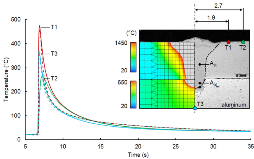
Fig. 15. Computed versus measured temperature cycles. Exemplary for regime 2 (Table 3). Solid lines – measurement, dashed lines – FEM. Distances to thermocouples are in mm.
