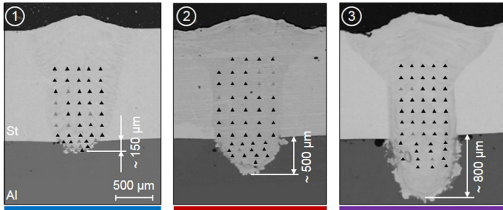
Fig. 7. Scheme of nanoindentation imprints in the investigated samples. Outliers are colored in grey. Imprints are not in scale. The samples are designated according to the corresponding welding regimes from Table 3.
