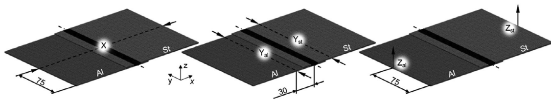
Fig. 18. Scheme of the evaluated distortions.
