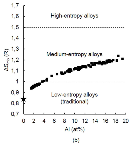
Fig. 21. Measured chemical composition (a) and calculated corresponding configurational entropy (b) of the weld metal as a function of Al concentration. Configurational entropy of stainless steel 304 ( \star ).
