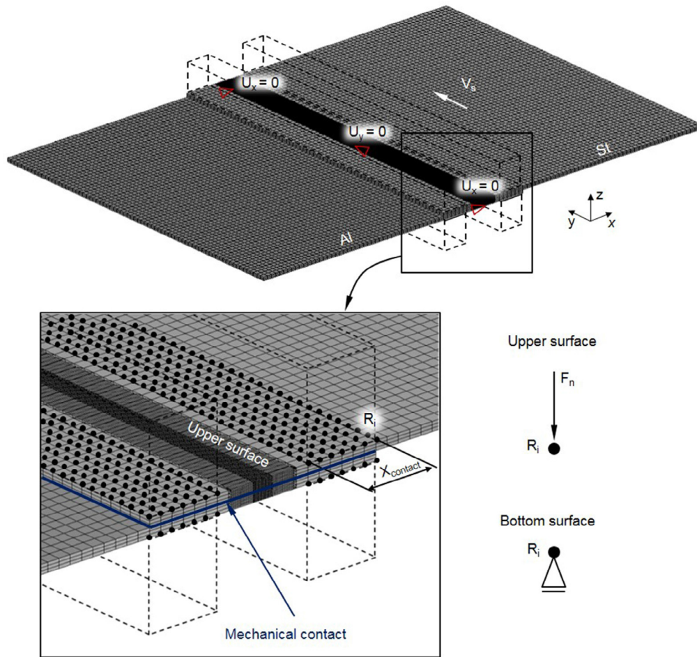
Fig. 13. Scheme of mechanical constraints during welding.
