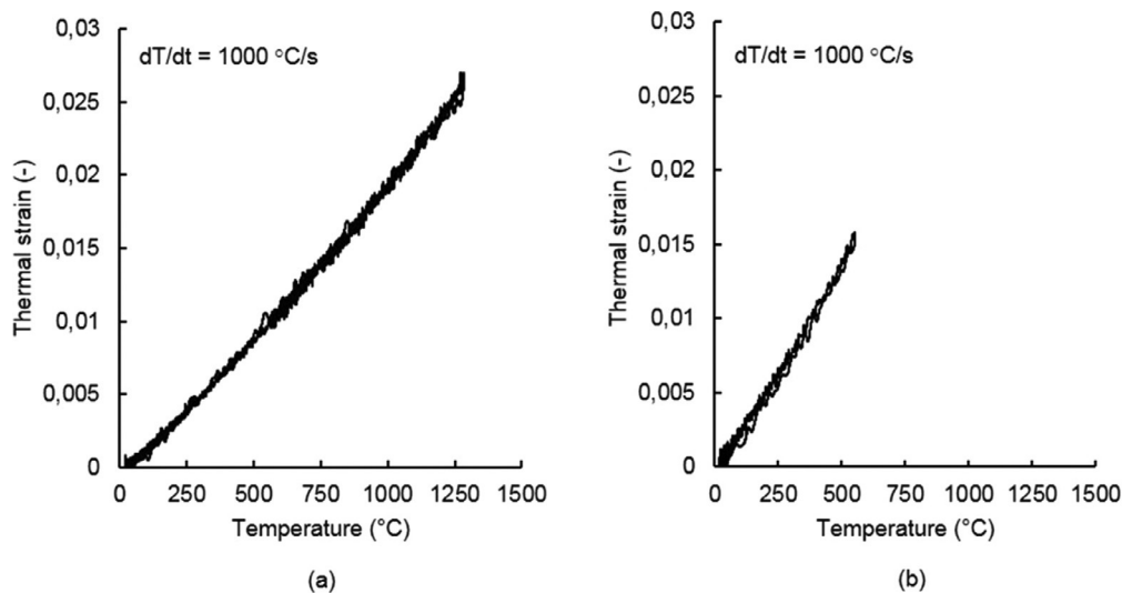
Fig. 4. Measured thermal expansion of 304 steel (a) and 6082-T6 aluminum alloy (b).
