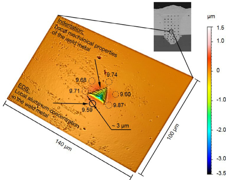
Fig. 6. The approach to determine the mechanical properties of the St-Al weld metal as a function of the aluminum concentration. Aluminum concentrations are given in at%.
