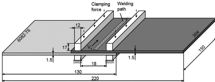
Fig. 1. Schematic illustration of welding trials.
