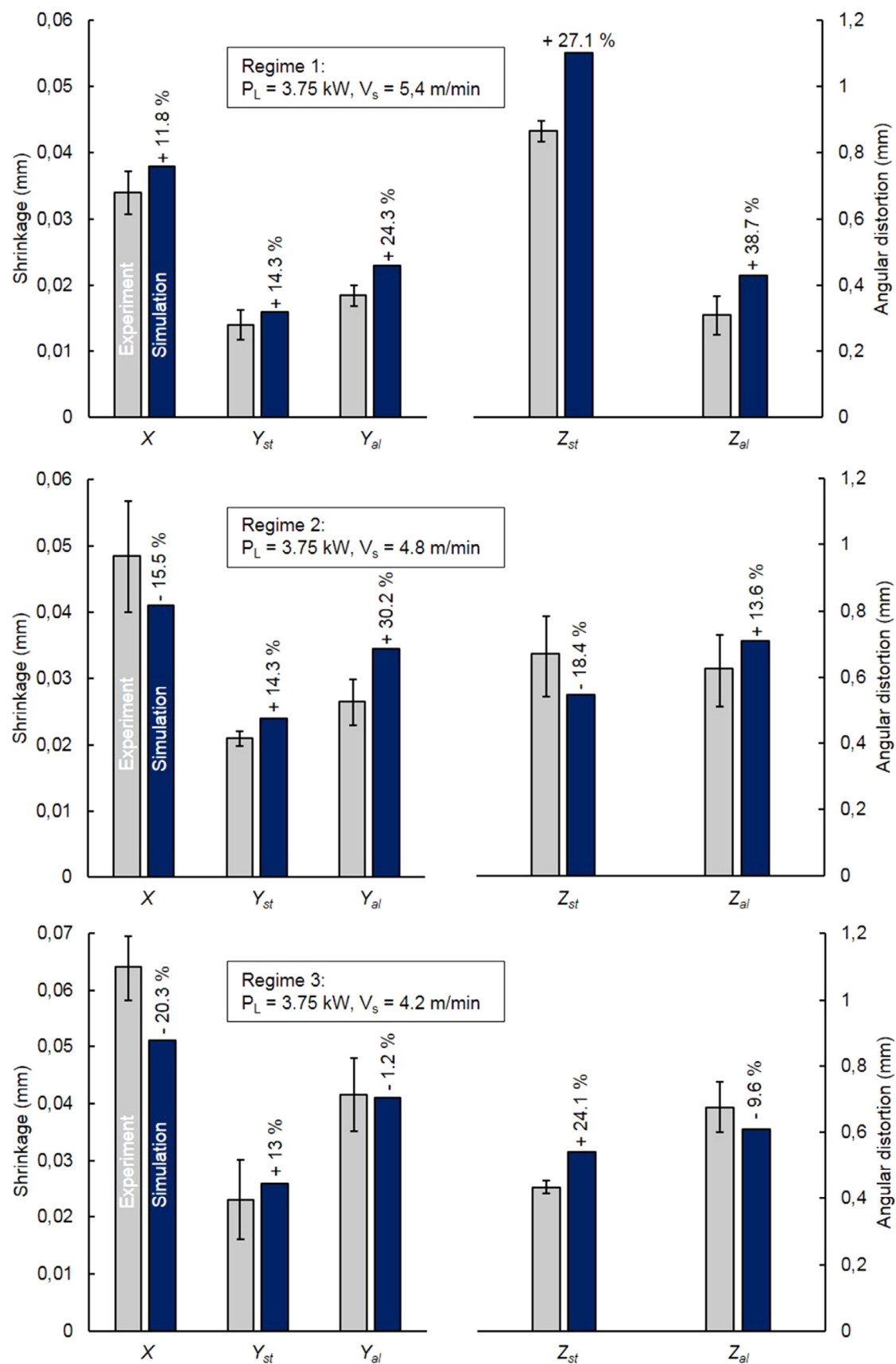
Fig. 19. Measured versus computed distortions.
