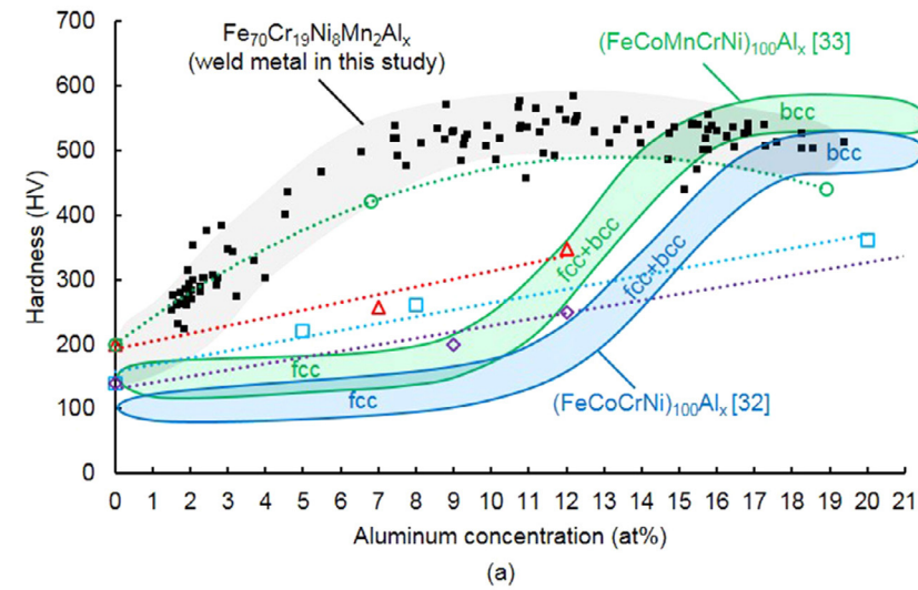
Fig. 20. Hardness (a) and yield strength (b) versus Al concentration. Weld metal arose after mixing of aluminum with non-alloyed steel ( \square [18], \diamond [19], \triangle [1]) and stainless steel ( \blacksquare [current study], \circ [36]).
