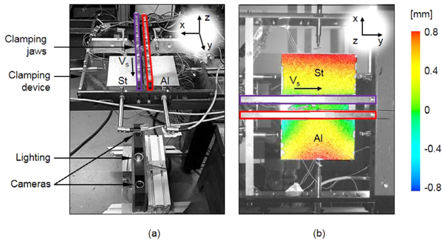
Fig. 2. Scheme of optical measurements (a). Measured residual out-of-plane displacements (b).
