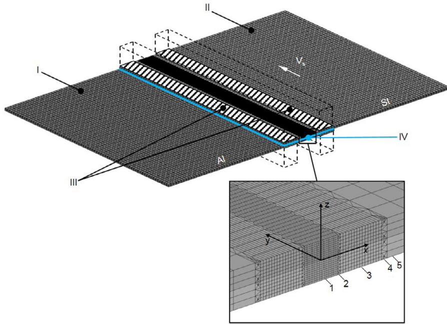
Fig. 12. Meshing strategy and boundary conditions. I, II – heat exchange with the ambient, III – heat losses into the clamping jaws, and IV – thermal contact between the sheets.
