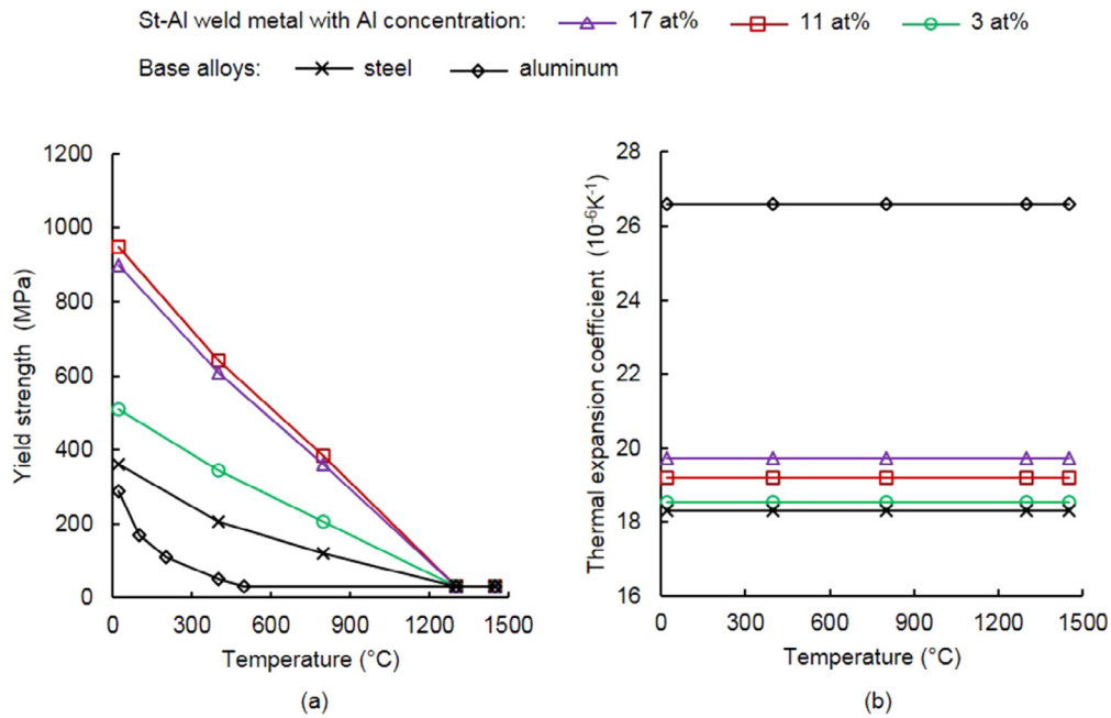
Fig. 11. Yield strength (a) and thermal expansion coefficient (b) of the St-Al weld metal as a function of aluminum concentration and temperature.
