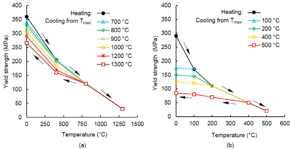
Fig. 5. Measured yield strength as a function of test and maximum temperatures of 304 steel (a) and 6082-T6 aluminum alloy (b).
