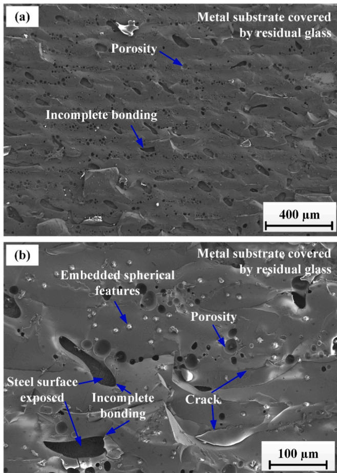
Fig. 3. Morphology of the separated interface showing residual glass layer on the metal substrate: (a) at low magnification; (b) at high magnification.
