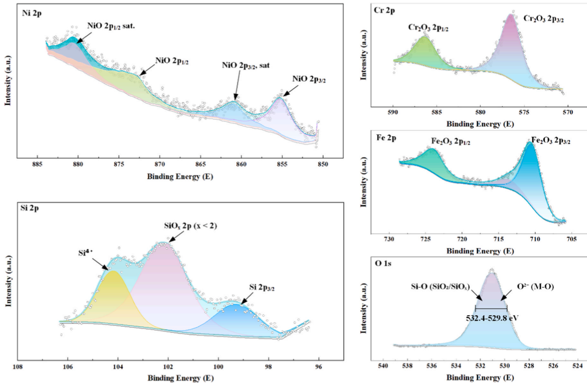
Fig. 7. XPS results at the joint interface.
