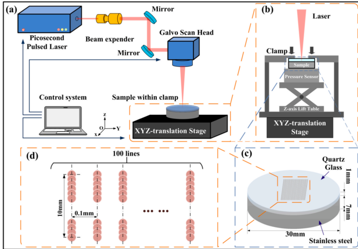
Fig. 1. Schematic diagram of ultrafast laser welding: (a) welding device; (b) fixture device; (c) samples and (d) scanning strategy.
