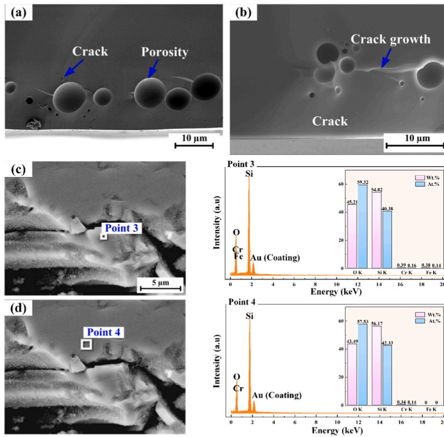
Fig. 6. Cracks induced by microstructural stresses at the interface: (a) micro-cracks; (b) crack growth; (c) and (d) quantitative EDS results near the cracks.
