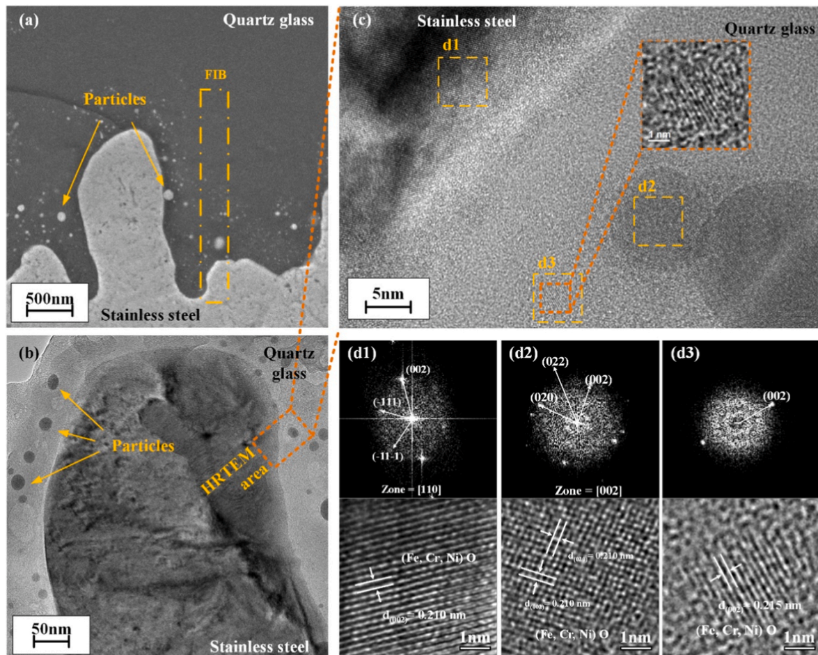
Fig. 8. TEM analysis at the stainless steel/quartz glass interface: (a) cross-sectional SEM of the interface with FIB location; (b) TEM of the interface with high resolution TEM (HRTEM) region; (c) HRTEM with three crystalline areas marked; (d) Crystallographic analysis of marked regions.
