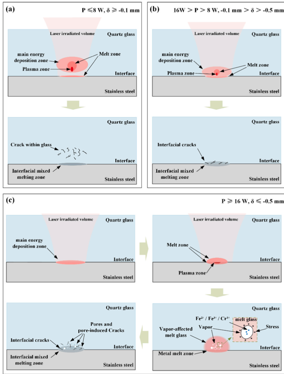
Fig. 10. Schematic diagram of defect formation mechanism: (a) defect formation under glass-volume-dominated energy deposition; (b) defect formation under glass-metal interfacial energy deposition; (c) defect formation under metal-surface-dominated energy deposition.
