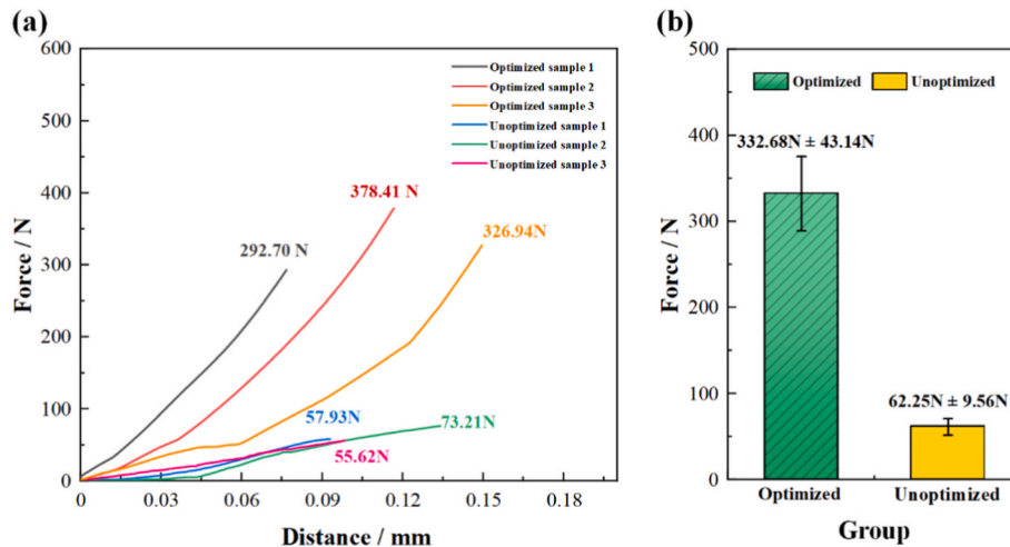
Fig. 12. Shear performance of best parameters: (a) load-displacement curves for three identical tests from optimized and unoptimized groups; (b) comparison of the mean maximum load.
