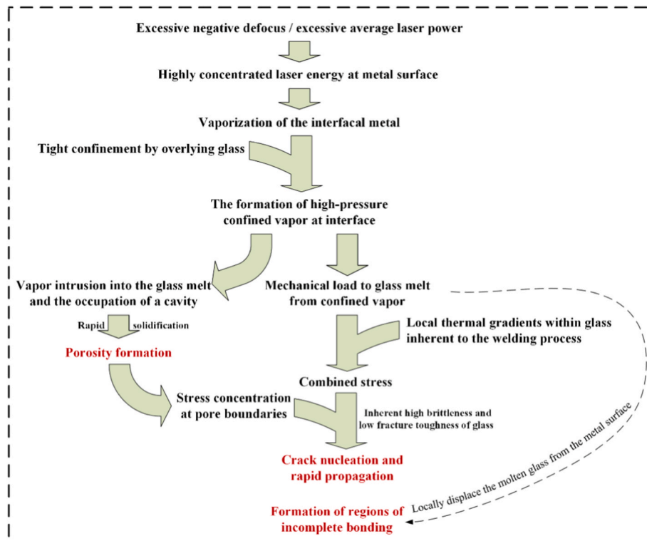
Fig. 11. Process model of defect formation.
