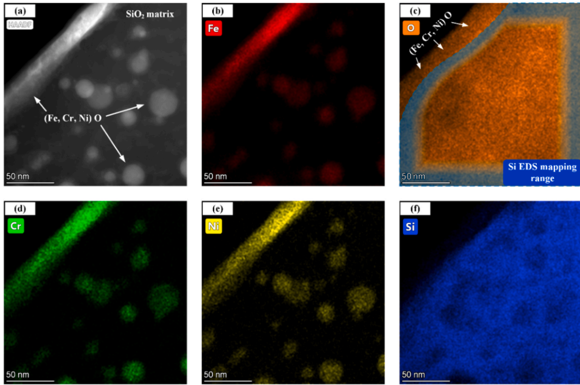
Fig. 9. Nanoscale elemental distribution across the interface by STEM-EDS mapping: (a) HAADF image of the interface and EDS mapping of (b) Fe, (c) O, (d) Cr, (e) Ni, (f) Si.
