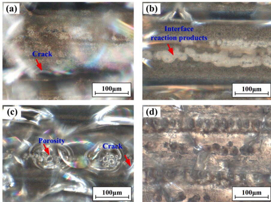
Fig. 2. Macroscopic morphology of the joint under different defocus conditions: (a) -0.1 \text{ mm} ; (b) -0.3 \text{ mm} ; (c) -0.5 \text{ mm} ; (d) -0.7 \text{ mm} .
