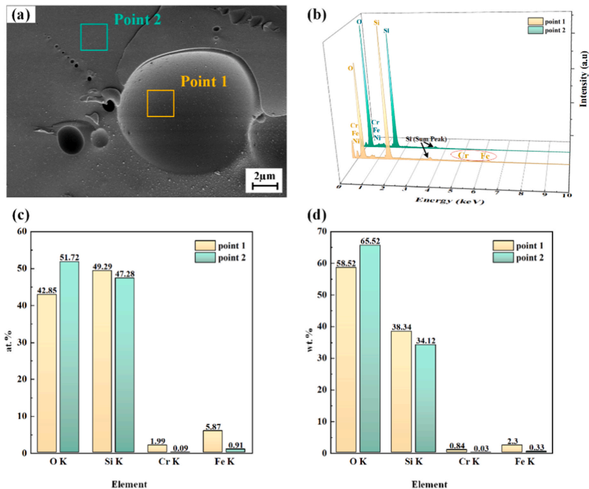
Fig. 5. EDS results at different positions on the glass fracture surface: (a) positions for EDS point analysis; (b) comparison of EDS spectra at the two positions; (c) elemental atomic ratio; (d) elemental weight ratio.
