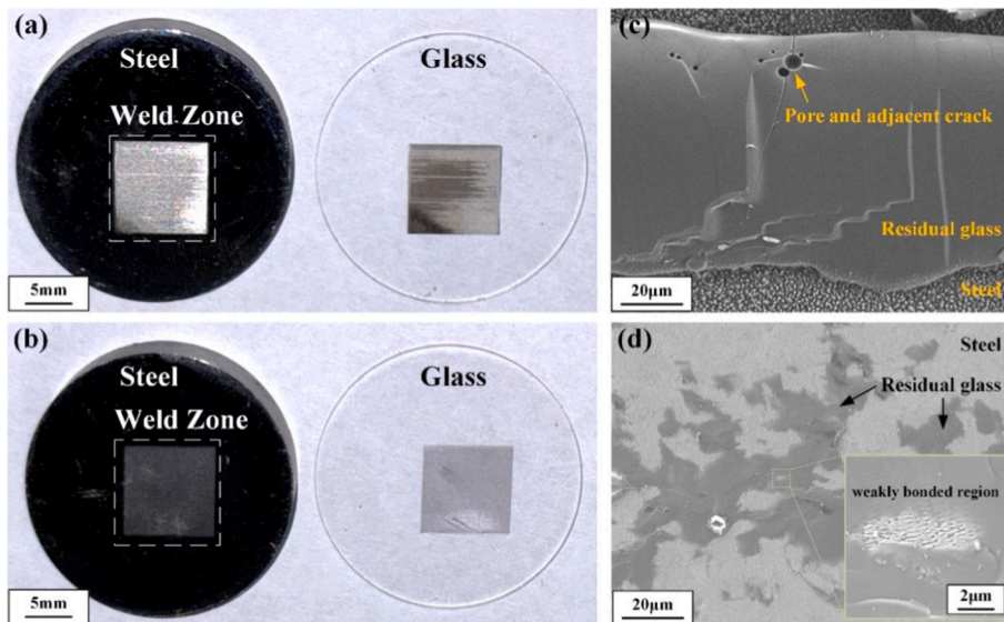
Fig. 13. Comparative analysis of fracture surface morphologies: macroscopic view of fracture surface from (a) unoptimized sample and (b) optimized sample; SEM micrograph of fracture surface from (c) unoptimized sample and (d) optimized sample.
