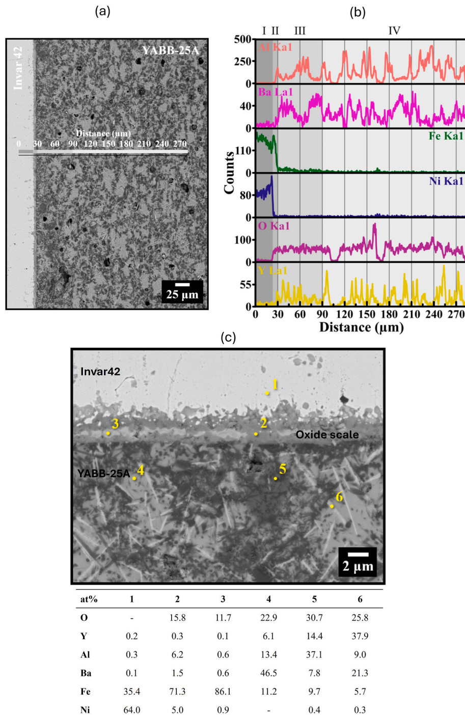
Fig. 10. (a) BSE cross-sectional micrograph of the Invar42/YABB-25A/ \text{Al}_2\text{O}_3 joined sample and (b) line-scan EDS analysis acquired along the line indicated in (a). (c) Higher magnification of FE-SEM image of the Invar42/oxide scale and oxide scale/YABB-25A sealant interfaces, together with the corresponding point EDS compositional analyses.
