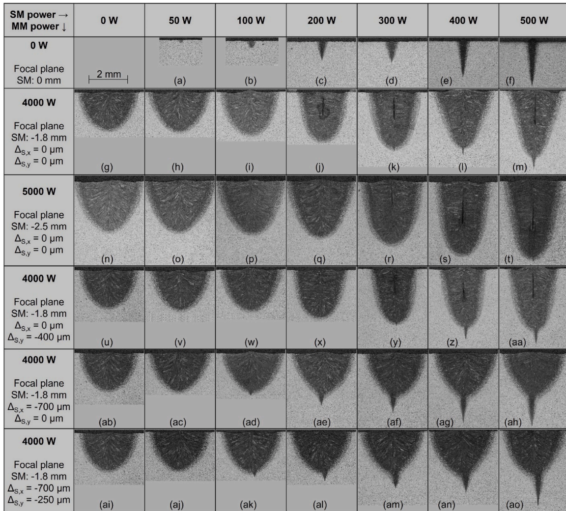
Fig. 10. Metallographic cross-sections.
