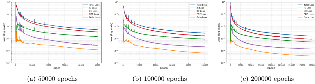
Fig. 9. Training loss of the PINN model for each epoch.
