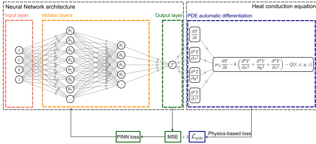
Fig. 1. Physics informed neural network model architecture.
