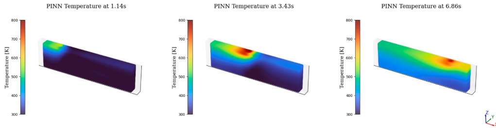
Fig. 5. 3D temperature field of the PINN model at three different time points.
