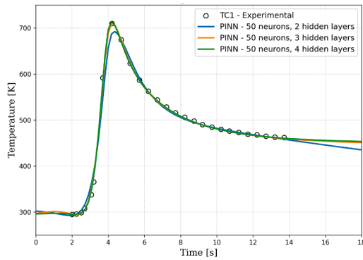
Fig. 14. Comparison of PINN model predictions at varying hidden layers with experimental data [28] at TC1 probe location.
