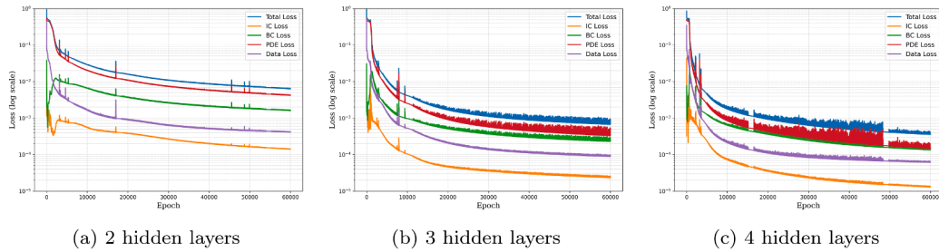
Fig. 13. Training loss of the PINN model for each hidden layer.
