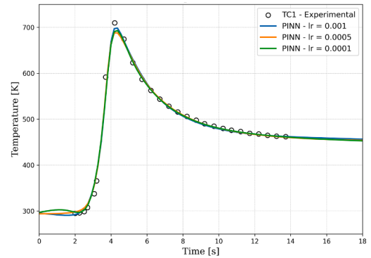
Fig. 8. Comparison of PINN model predictions at varying learning rates with experimental data [28] at TC1 probe location.
