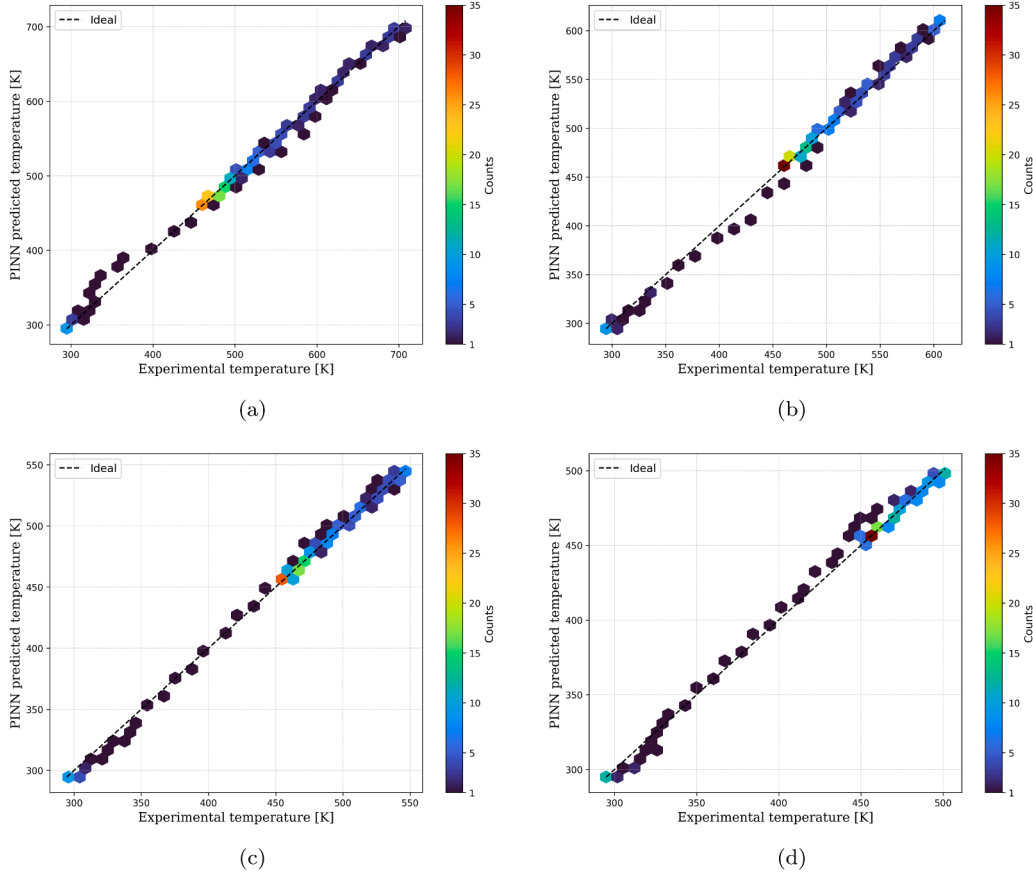
Fig. 6. Hexbin plots comparing PINN-predicted temperatures with experimental measurements at thermocouple locations ((a)-TC1, (b)-TC2(c)-TC3(d)-TC4. The dashed diagonal line indicates the ideal y = x relationship.
