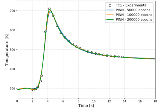
Fig. 10. Comparison of PINN model predictions at varying epoch sizes with experimental data [28] at TC1 probe location.
