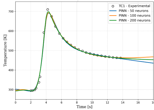
Fig. 12. Comparison of PINN model predictions at varying neuron sizes with experimental data [28] at TC1 probe location.
