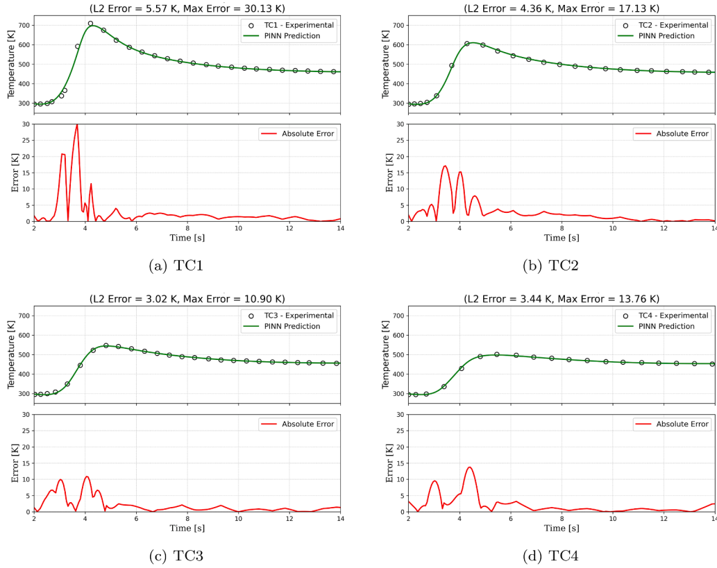
Fig. 4. Comparison of PINN model predictions vs. experimental data [28] at each probe location.
