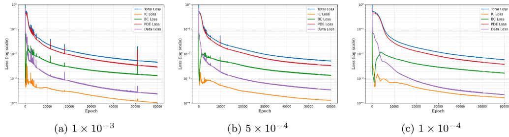
Fig. 7. Training loss of the PINN model for each learning rate.
