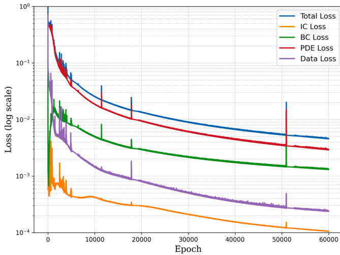
Fig. 3. Training loss of the PINN model.
