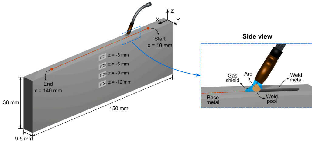
Fig. 2. Sample dimensions, weld line and thermocouple locations. Adapted from [28].
