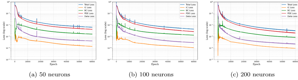
Fig. 11. Training loss of the PINN model for each neuron size.
