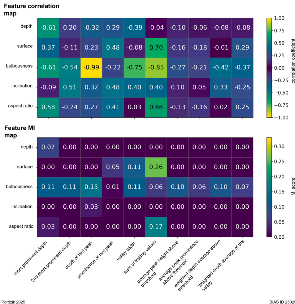
Fig. 19. Feature mapping between keyhole geometry features and OCT histogram features for a welding process carried out at a laser power of 6 kW by means of correlation analysis (top) and MI analysis (bottom).
