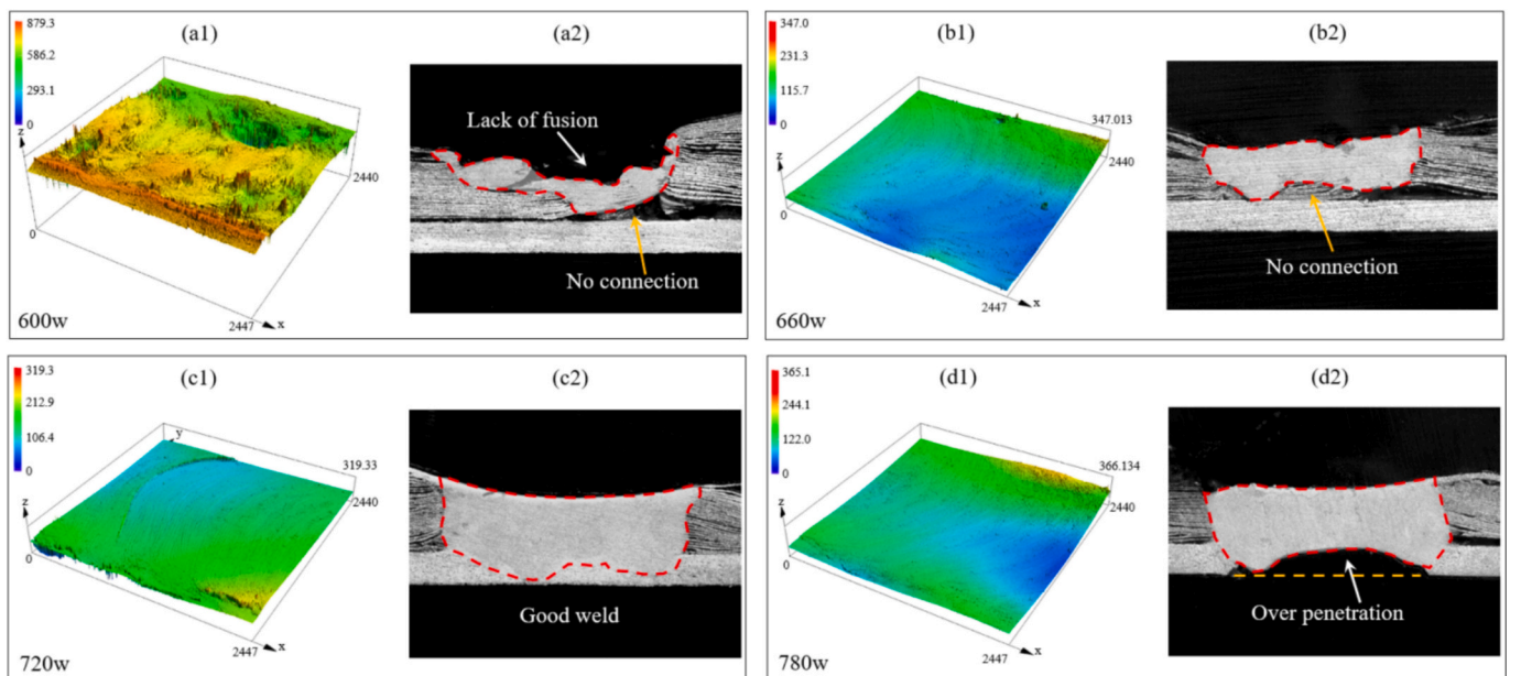
Fig. 13. Comparative analysis of weld cross-section and surface topography under different laser powers.
