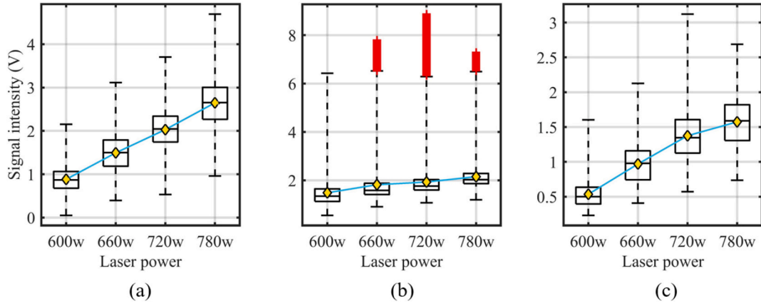
Fig. 6. Box plot of optical radiation signals during laser welding at various laser powers. (a) P-Signal. (b) R-Signal. (c) T-Signal.
