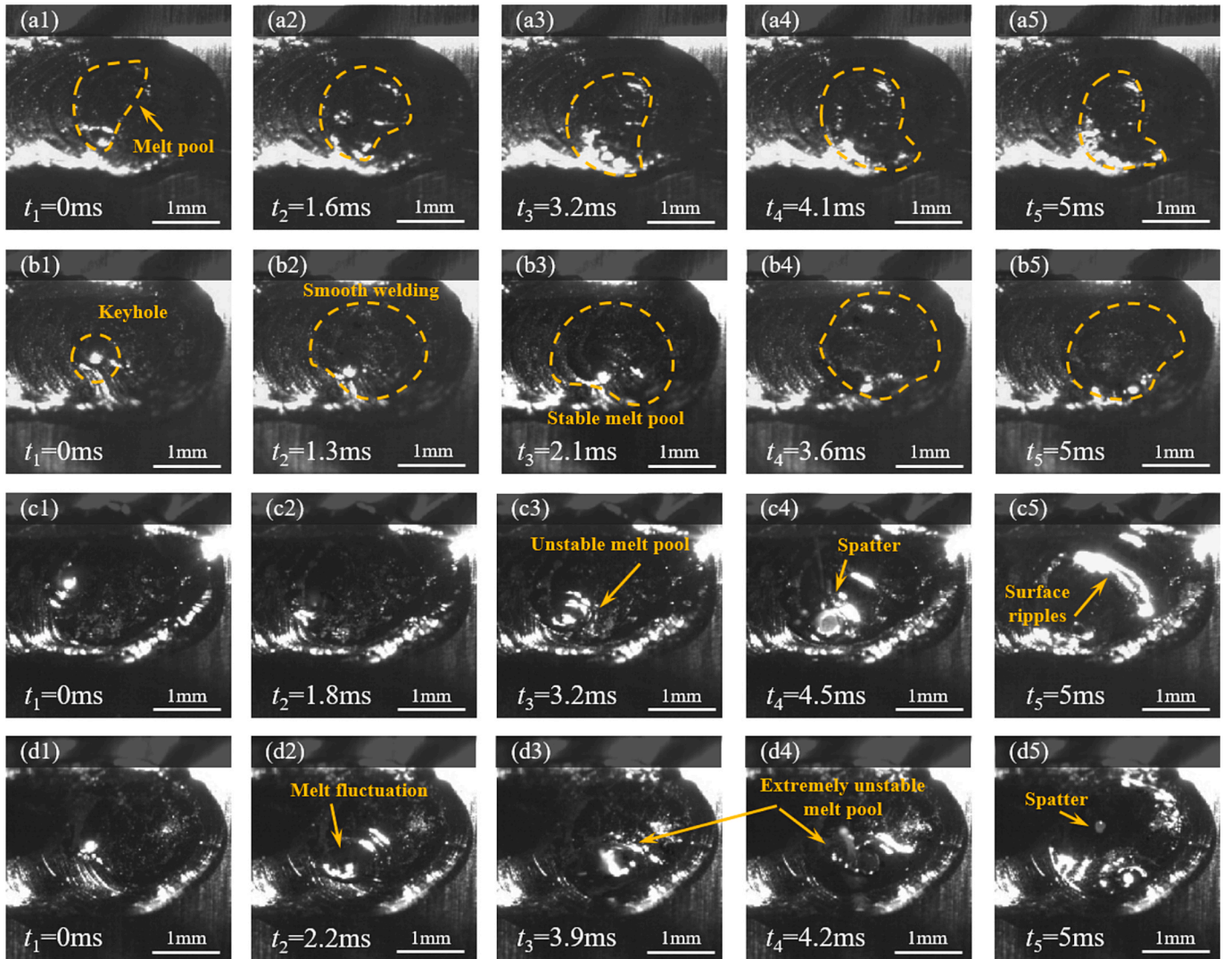
Fig. 7. Evolutionary behavior of the melt pool at different powers. (a) Laser power = 600w. (b) Laser power = 660w. (c) Laser power = 720w. (d) Laser power = 780w.
