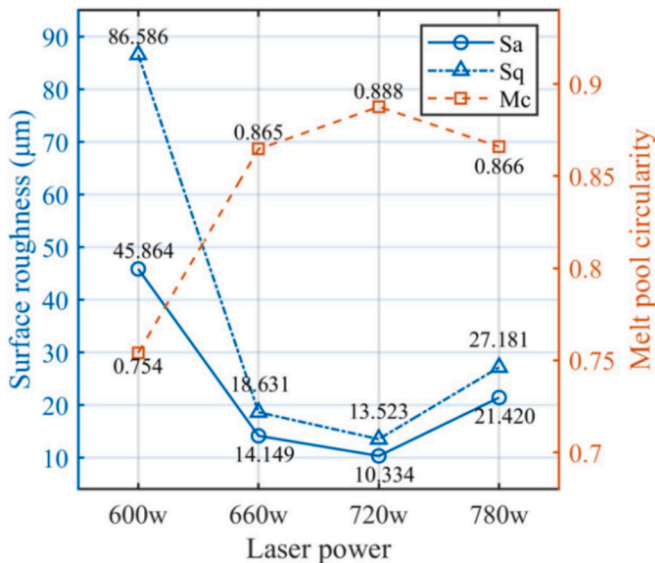
Fig. 14. Variation of surface roughness and melt pool circularity with laser power.
