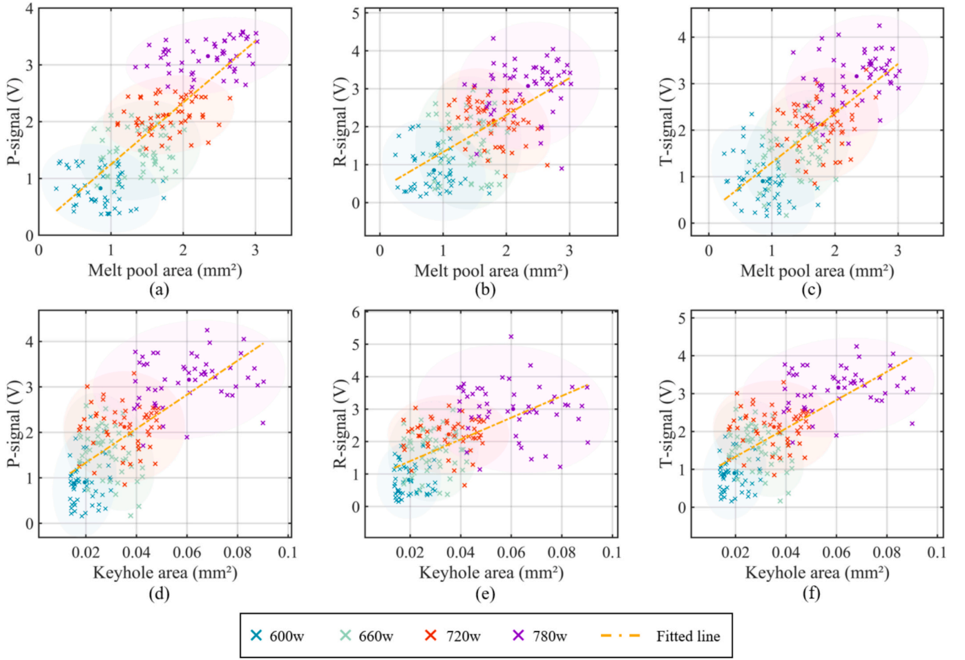
Fig. 15. Correlation graphs between measured weld dimensions and signals for photodiodes.
