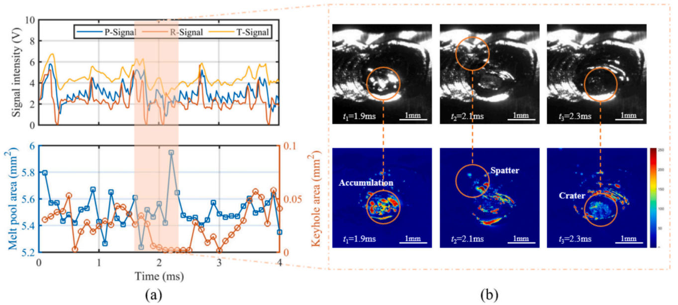
Fig. 12. The optical signals and related high-speed images at a melt ejection case. (a) Raw signals. (b) Relative high-speed images in ejection process.
