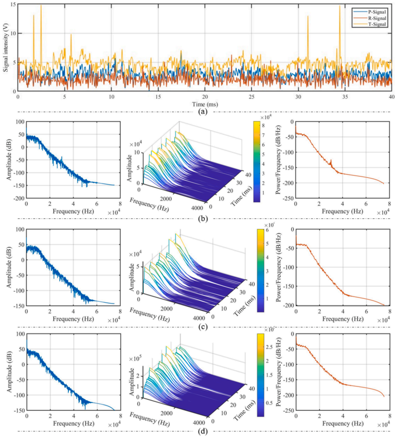
Fig. 9. Characterization of optical radiation signals. (a) Raw signal. (b) Frequency domain characteristics of the P-Signal. (c) Frequency domain characteristics of the R-Signal. (d) Frequency domain characteristics of the T-Signal.
