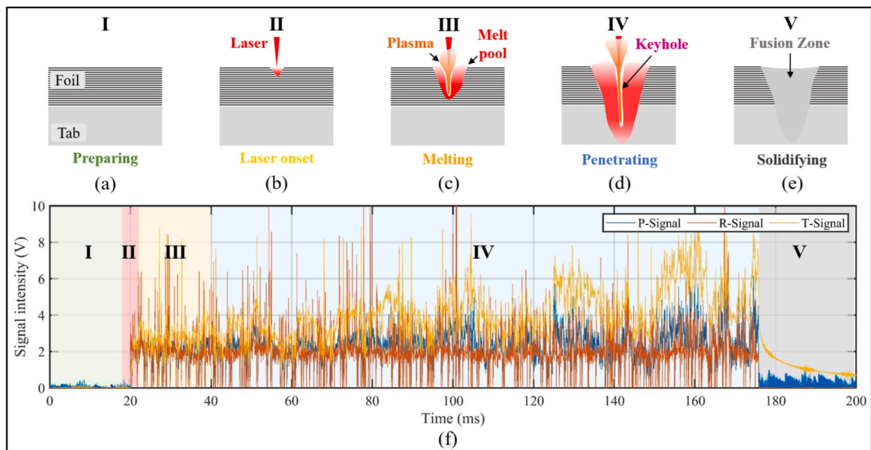
Fig. 5. Schematic of the laser welding stage classification and typical photoelectric signals for each stage. (a) Stage I (Preparation): Laser off, no energy input to the workpiece. (b) Stage II (Activation): Laser on, beam contacts the material surface, initial heat absorption. (c) Stage III (Melting): Material melts, shallow pool forms with continued laser energy. (d) Stage IV (Penetration): Heat conducts inward, pool deepens, material penetrated. (e) Stage V (Solidification): Welding complete, workpiece cools or undergoes post-treatment. (f) Three-band optical radiation signals for each stage.
