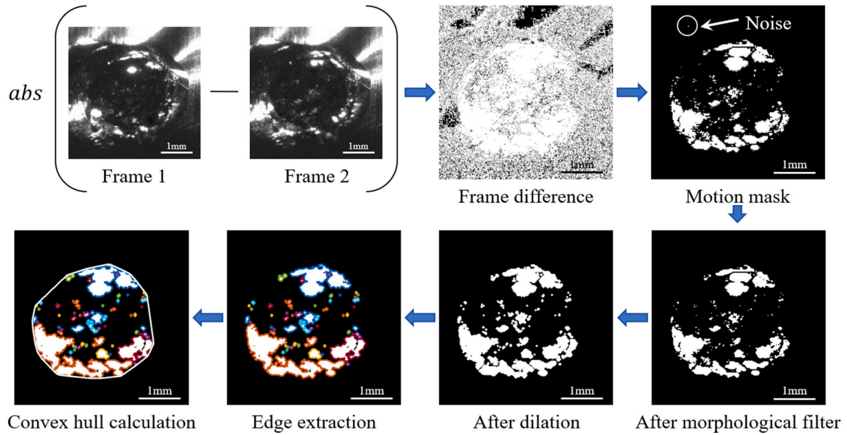
Fig. 3. Melt pool extraction process based on frame difference and convex hull calculation.
