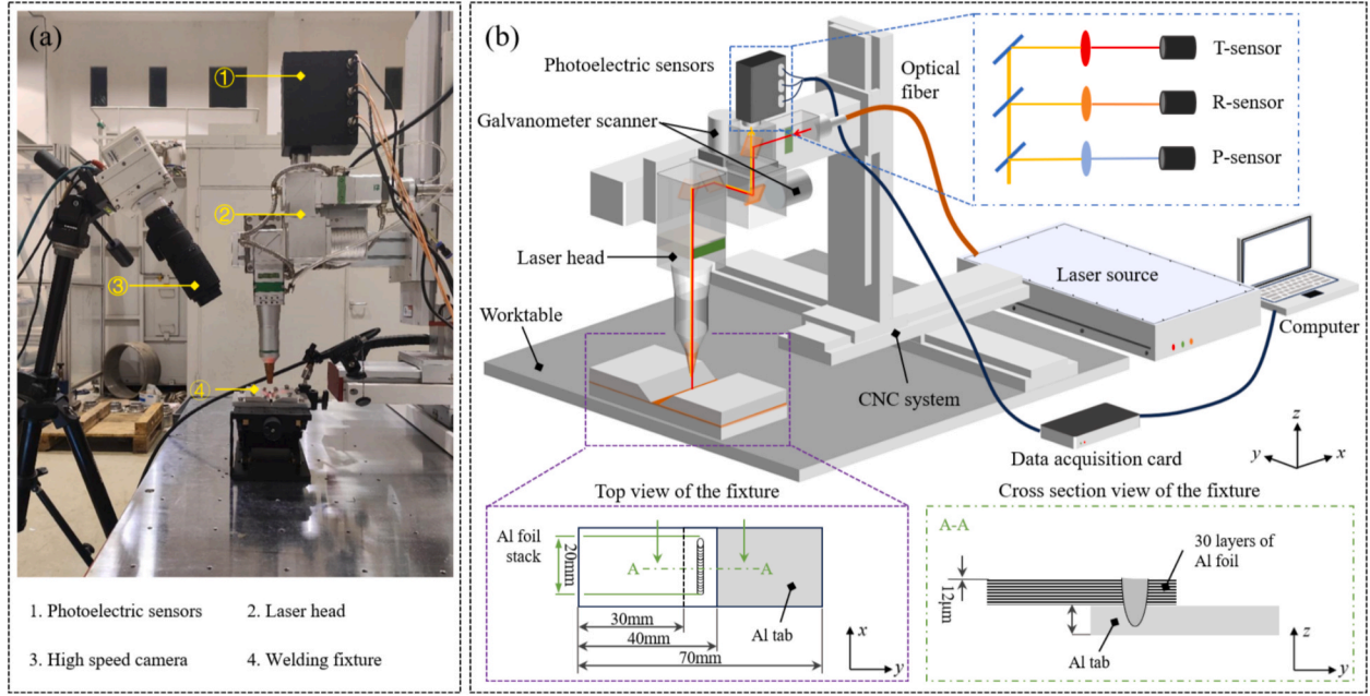
Fig. 1. View of the experimental platform.
