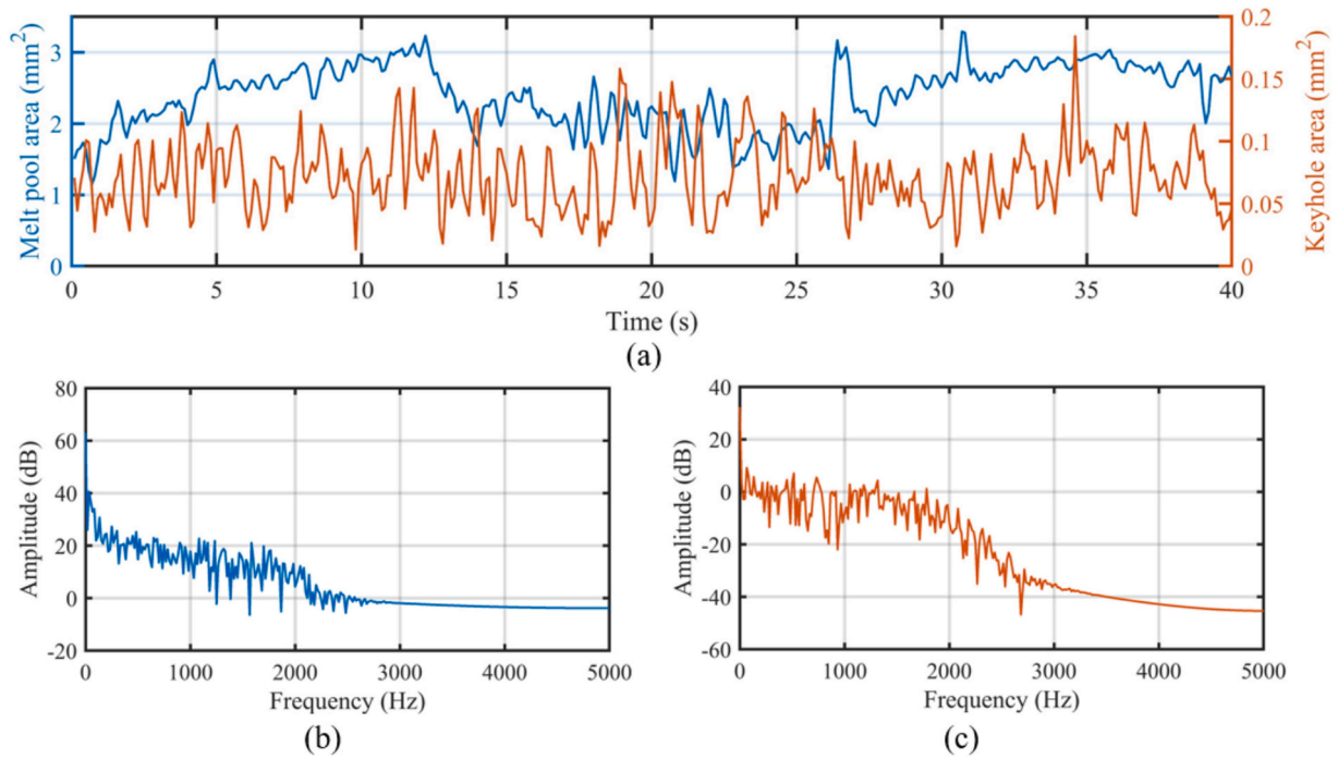
Fig. 10. Melt pool and keyhole area dynamics and frequency domain characteristics. (a) Time variation of melt pool and keyhole area. (b) Frequency domain characteristics of melt pool. (c) Frequency domain characteristics of keyhole.
