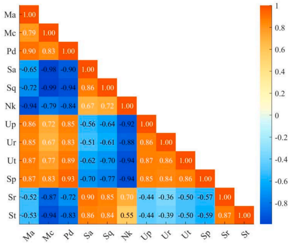
Fig. 16. Correlation matrix between weld features (Ma, Mc, Pd, Sa, Sq, and Nk) and signals features (Up, Ur, Ut, Sp, Sr and St).
