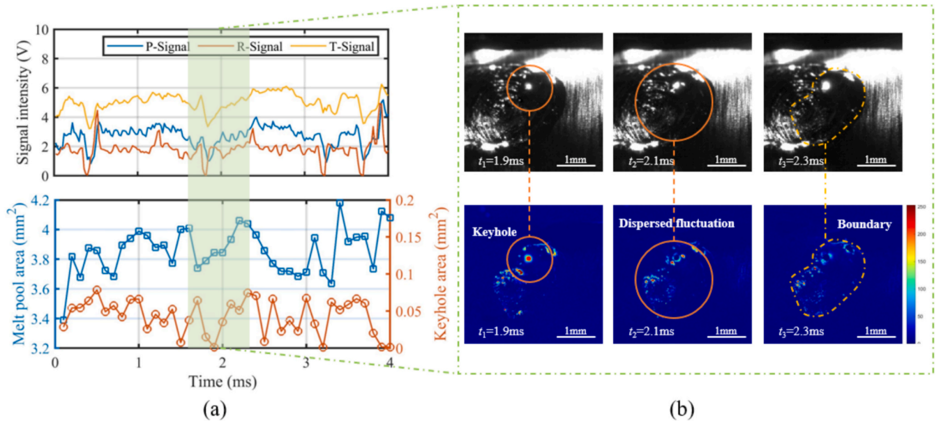
Fig. 11. The optical signals and related high-speed images in a typical slight oscillation situation. (a) Raw signals. (b) High-speed image at a slight oscillation point.
