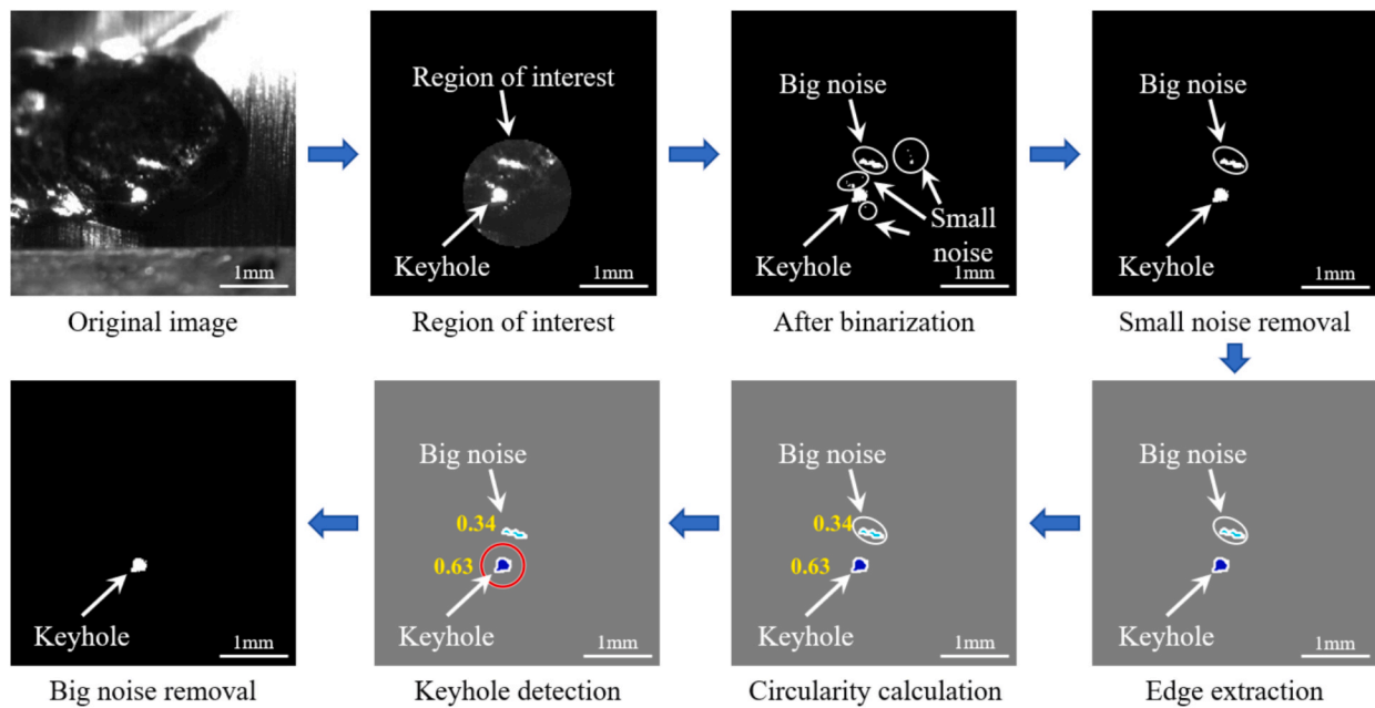
Fig. 4. Keyhole extraction algorithm based on welding trajectory tracking and morphological calculations.
