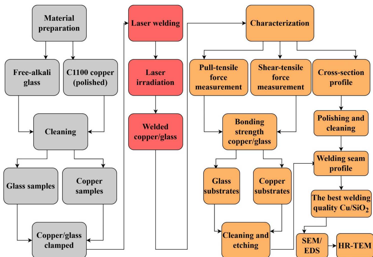
Fig. 1 Flowchart depicting the experimental process employed in this study.
