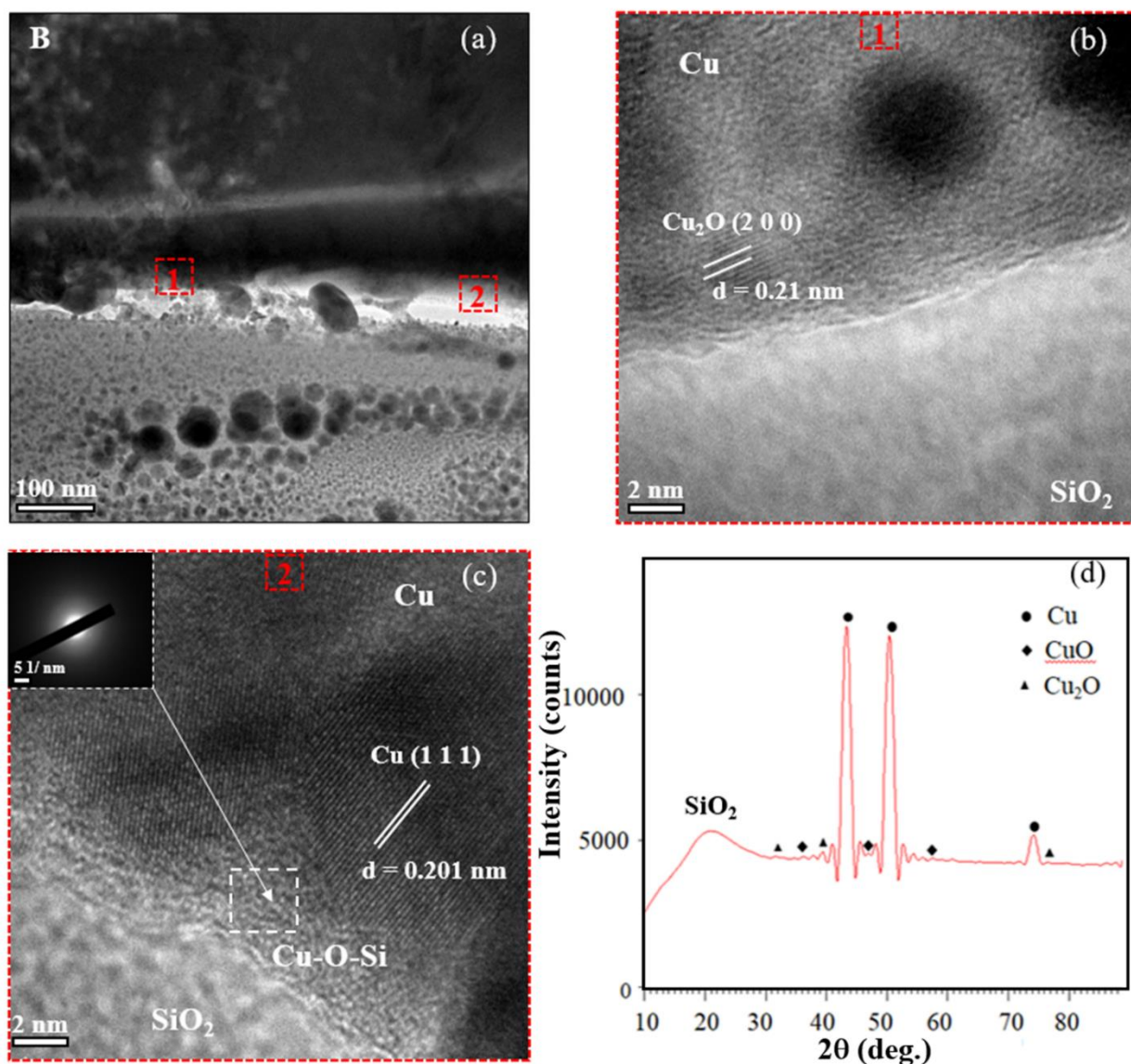
Fig. 8 Interfacial TEM images and XRD analysis. (a) TEM image focusing on the interfacial region around B, as indicated in Fig. 7 (b). (b) HR-TEM image of Area 1, enclosed by a red-dashed box labeled 1 in (a), for observing interfacial phase configurations. (c) HR-TEM image of Area 2, enclosed by the red-dashed box labeled 2 in (a), for observing interfacial phase configurations. (d) XRD patterns of the spotted Cu/SiO 2 weld interface.
