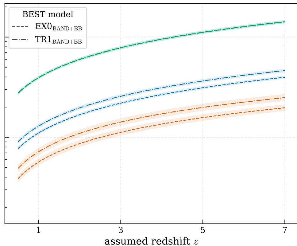
GRB140206B
