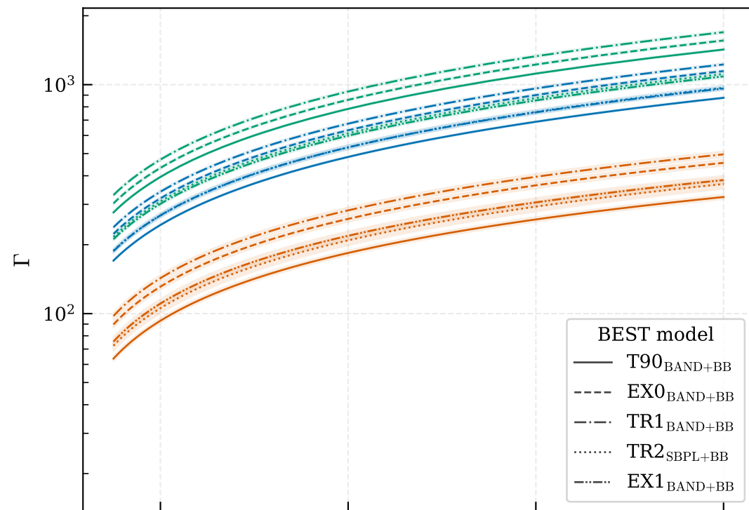
GRB131014A
