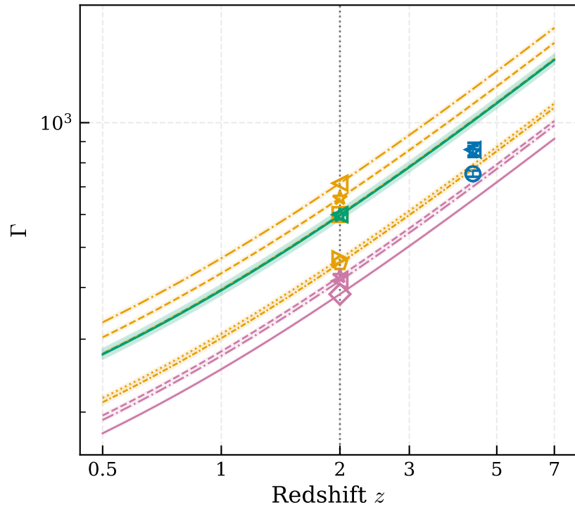
Lorentz factor \Gamma (at Y=1 ; \Gamma \propto Y^{1/4} )
