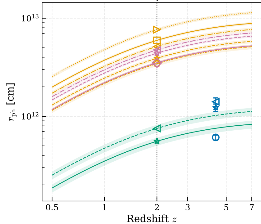
Photospheric radius r_{\text{ph}} (at Y=1 ; r_{\text{ph}} \propto Y^{1/4} )
