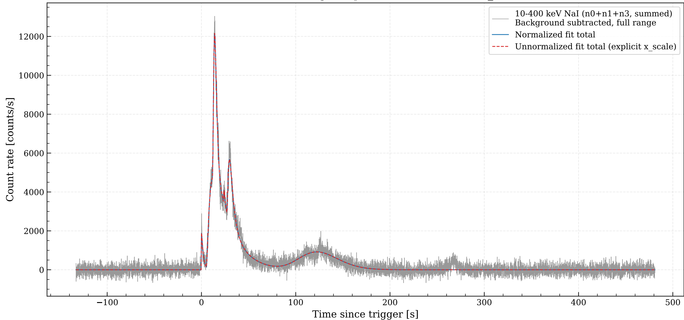
GRB140206B: full-range fit, pulse 6 re-seeded to (A, t_s, 1, 1)
