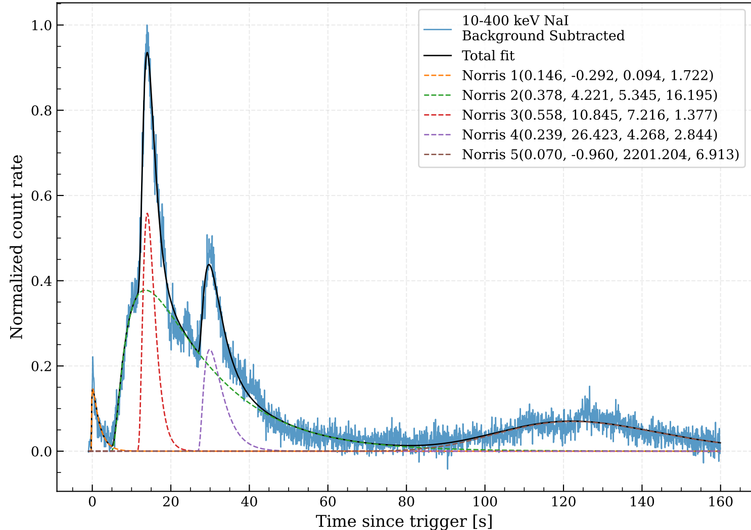
GRB140206B SIMPLE window-sensitivity check: narrow_1_160 [-1, 160] s
