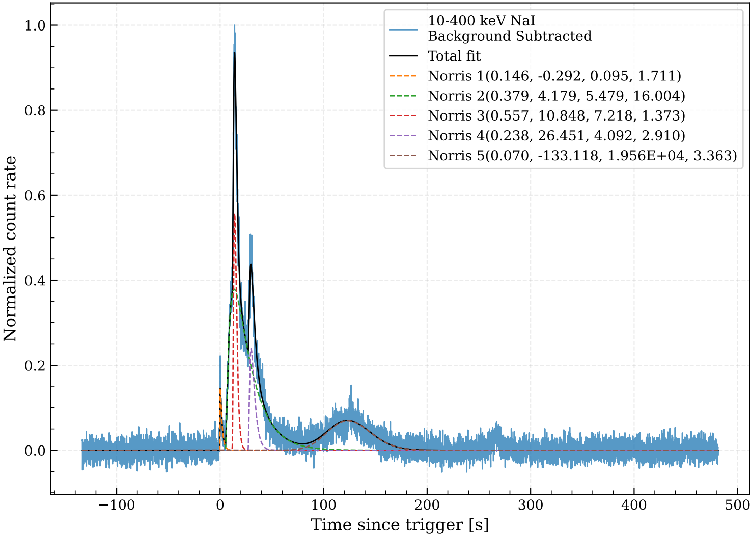
GRB140206B SIMPLE window-sensitivity check: widest_full_range [-133.184, 481.152] s
