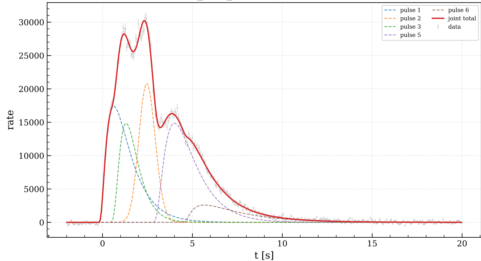
GRB231129C_joint_5pulse: joint 5-pulse 3-param fit
