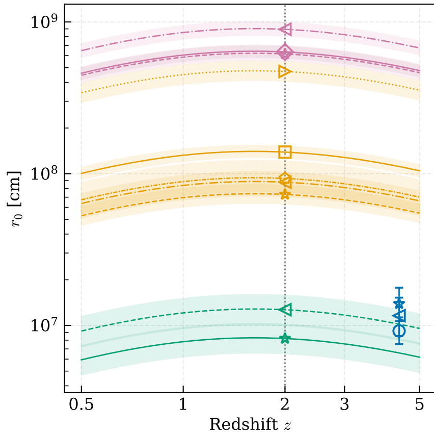
Base radius r_0 (at Y=1 ; r_0 \propto Y^{-3/2} )
