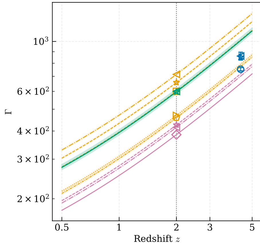
Lorentz factor \Gamma (at Y=1 ; \Gamma \propto Y^{1/4} )
