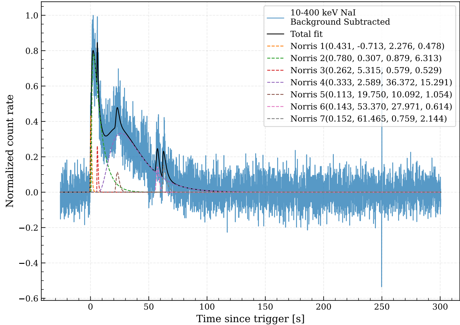
GRB080916C SEVEN-pulse window-sensitivity check: widest_full_range [-25.92, 300.608] s
