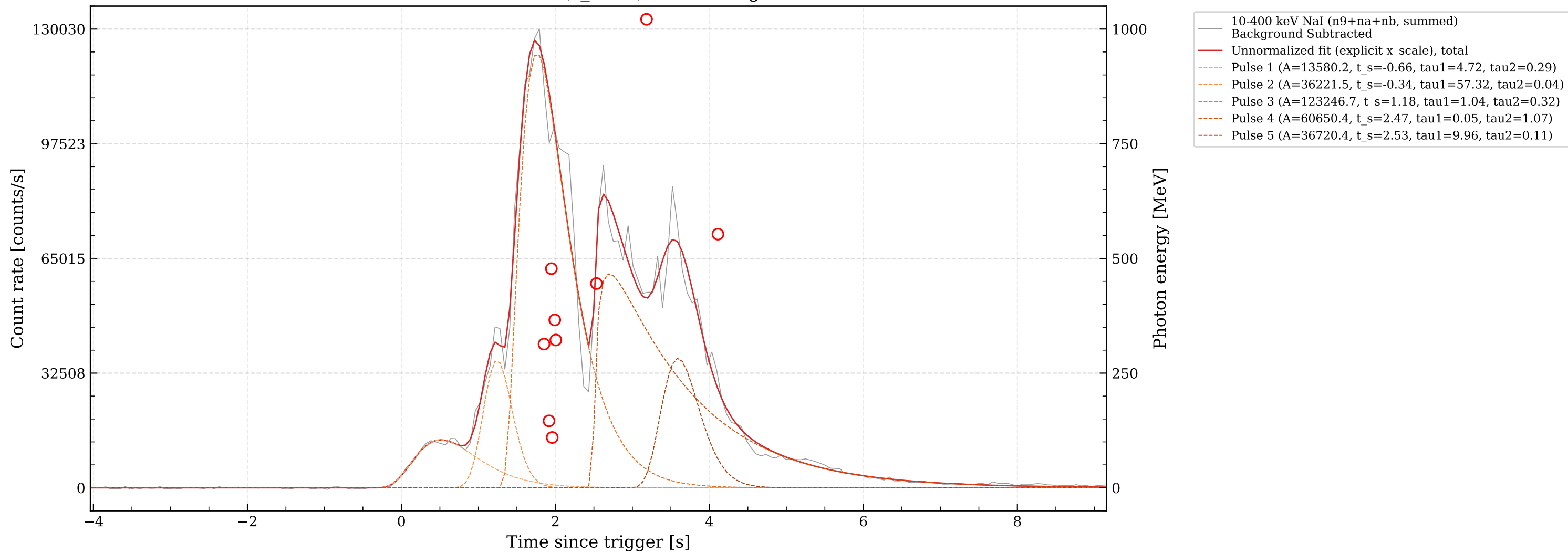
GRB131014A: unnormalized (x_scale) fit, full range -135.9-478.4s
