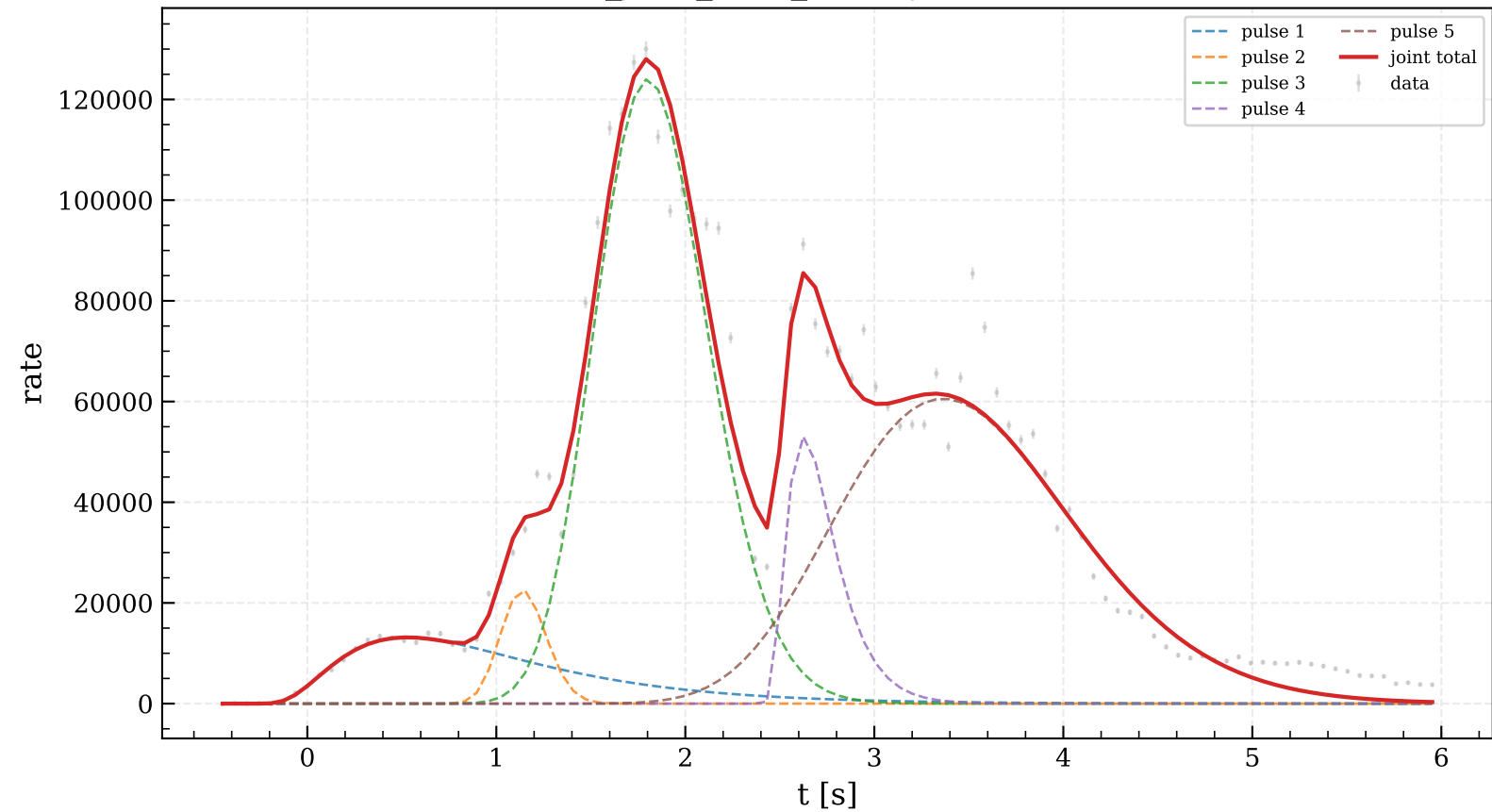
GRB131014215_joint_from_hints: joint 5-pulse 3-param fit
