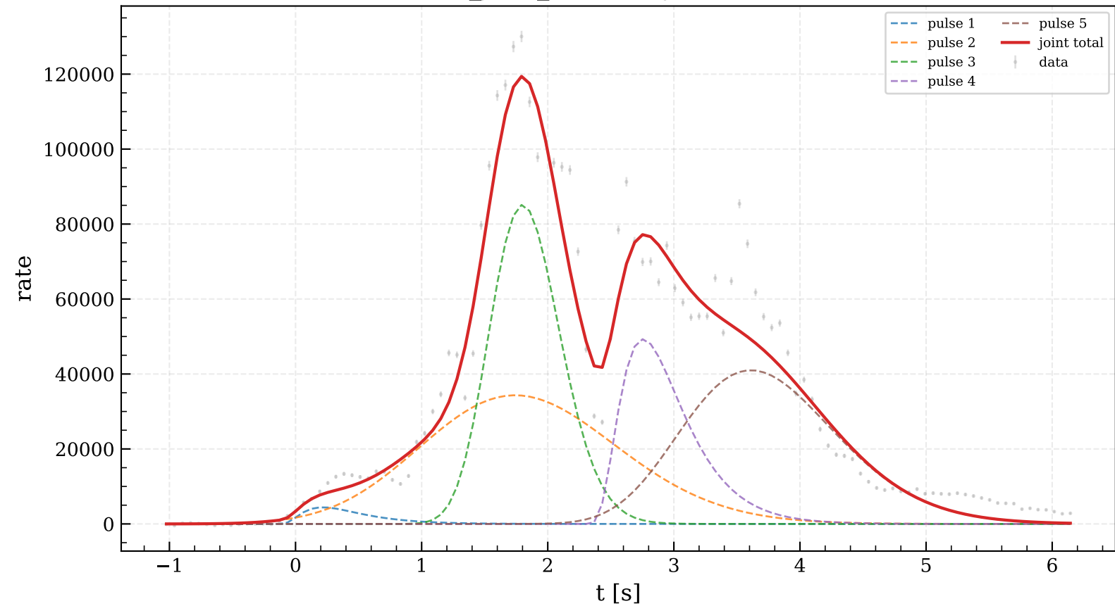
GRB131014215_joint_fullspan: joint 5-pulse 3-param fit
