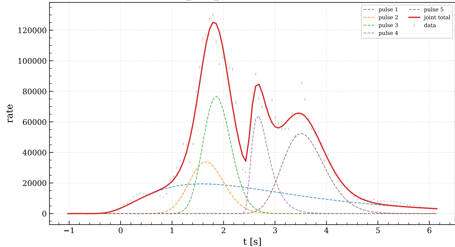
GRB131014215_joint_goldilocks: joint 5-pulse 3-param fit
