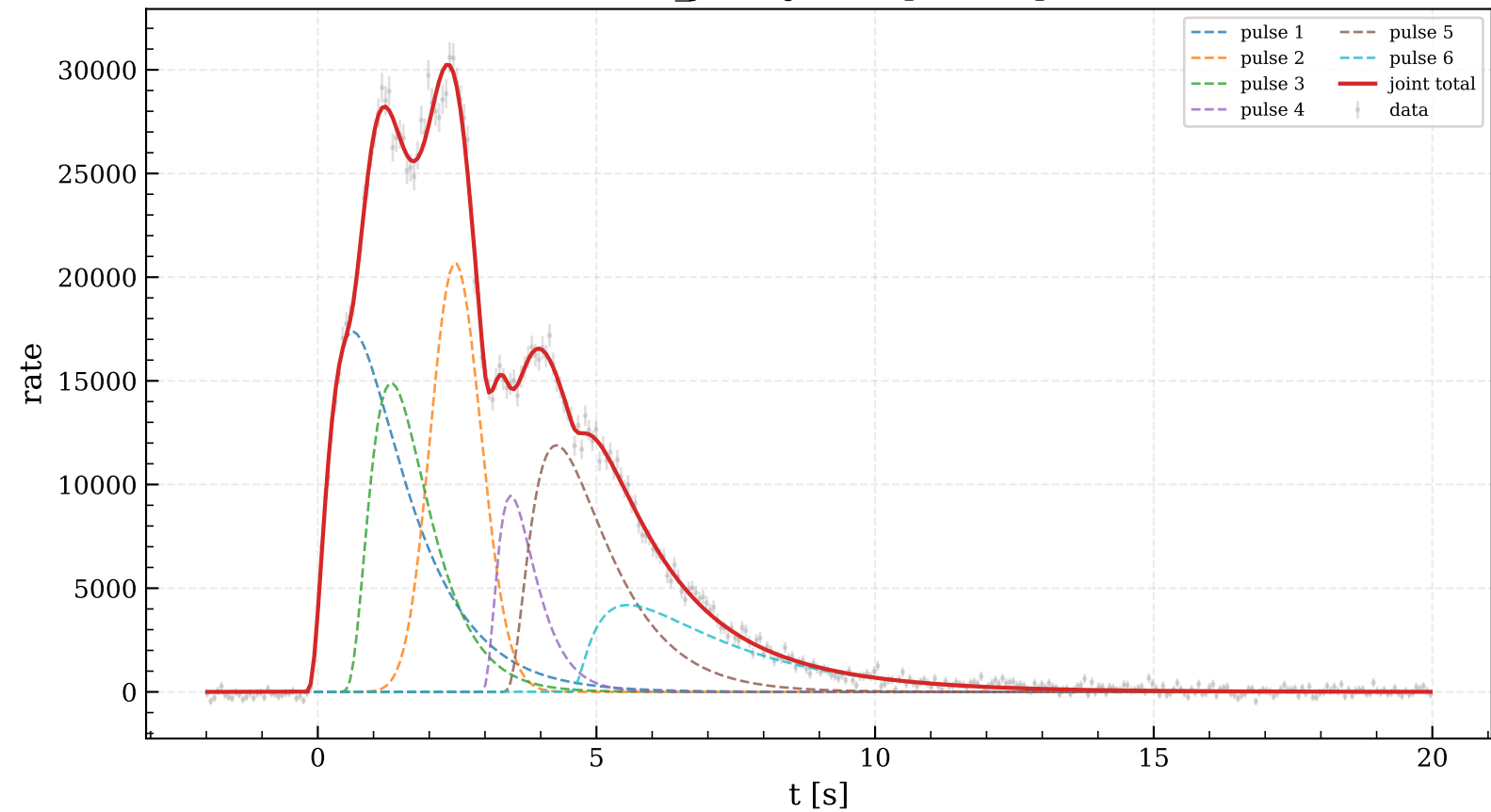
GRB231129C_joint: joint 6-pulse 3-param fit
