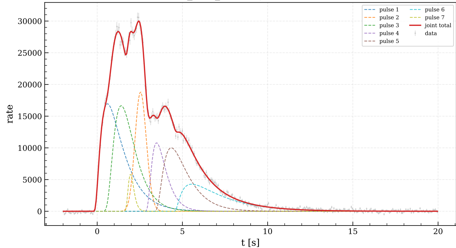
GRB231129C_joint_7pulse: joint 7-pulse 3-param fit
