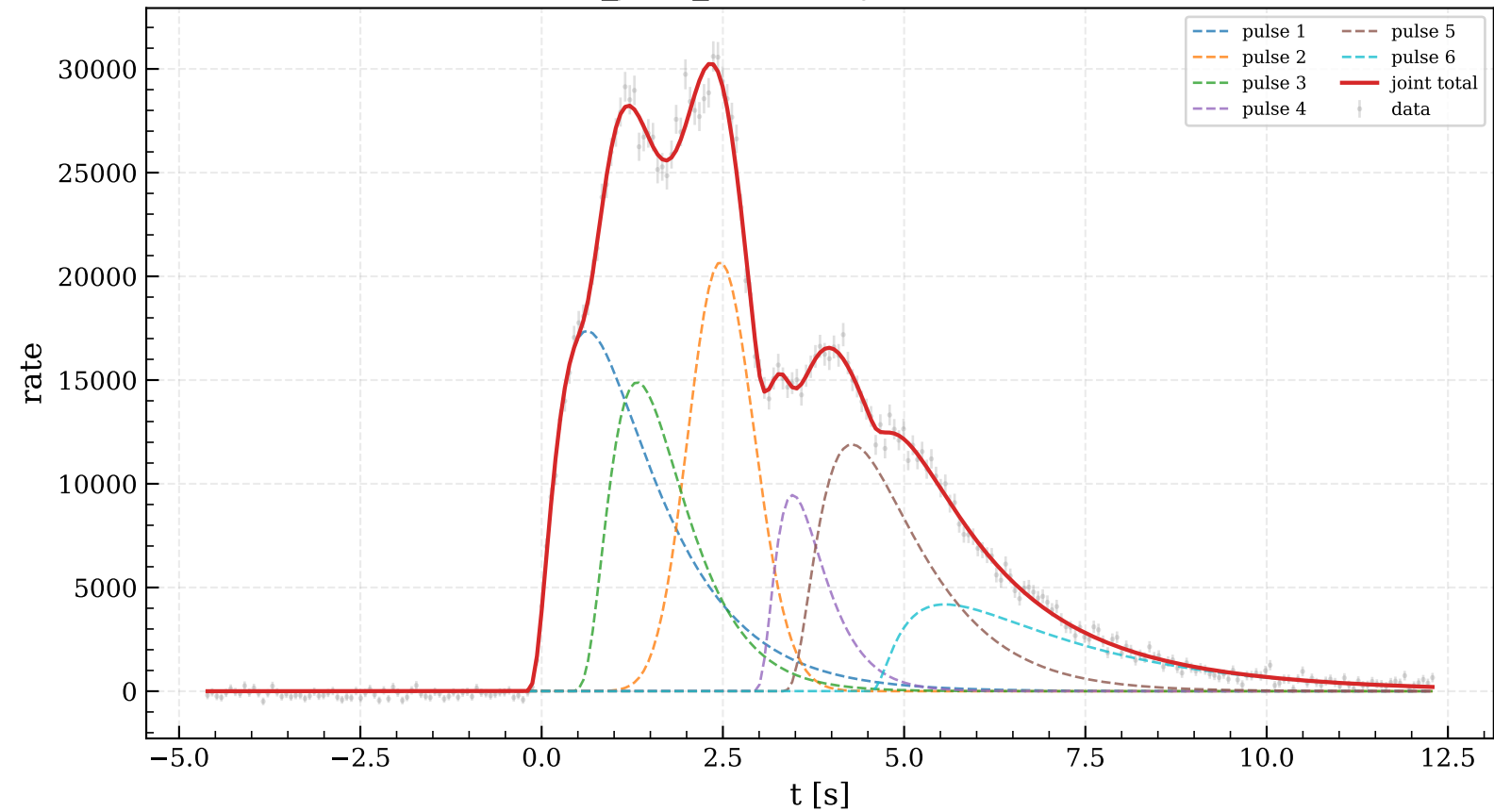
GRB231129C_joint_fullspan: joint 6-pulse 3-param fit
