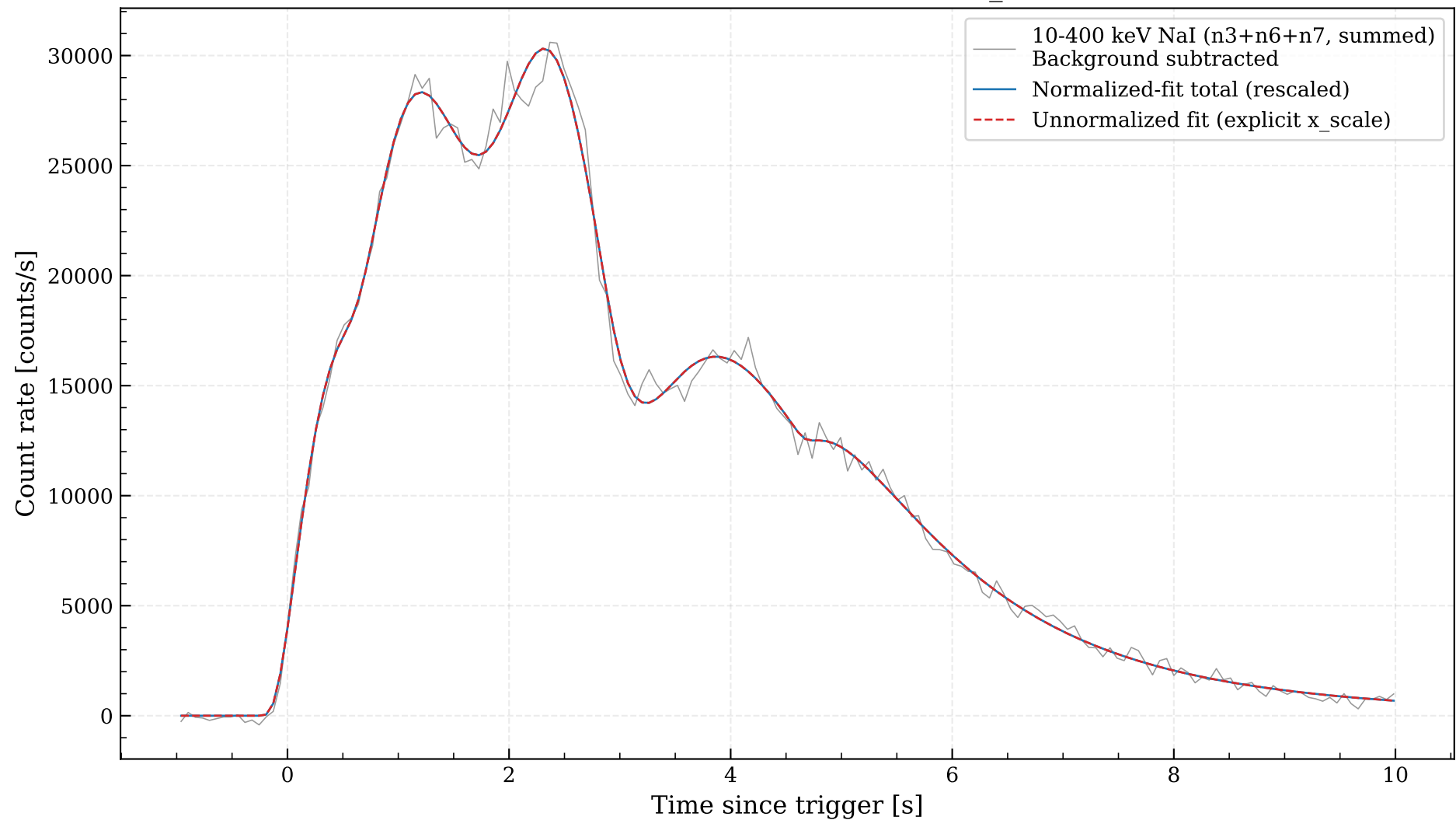
GRB231129C: normalized vs. unnormalized (x_scale) Norris fit
