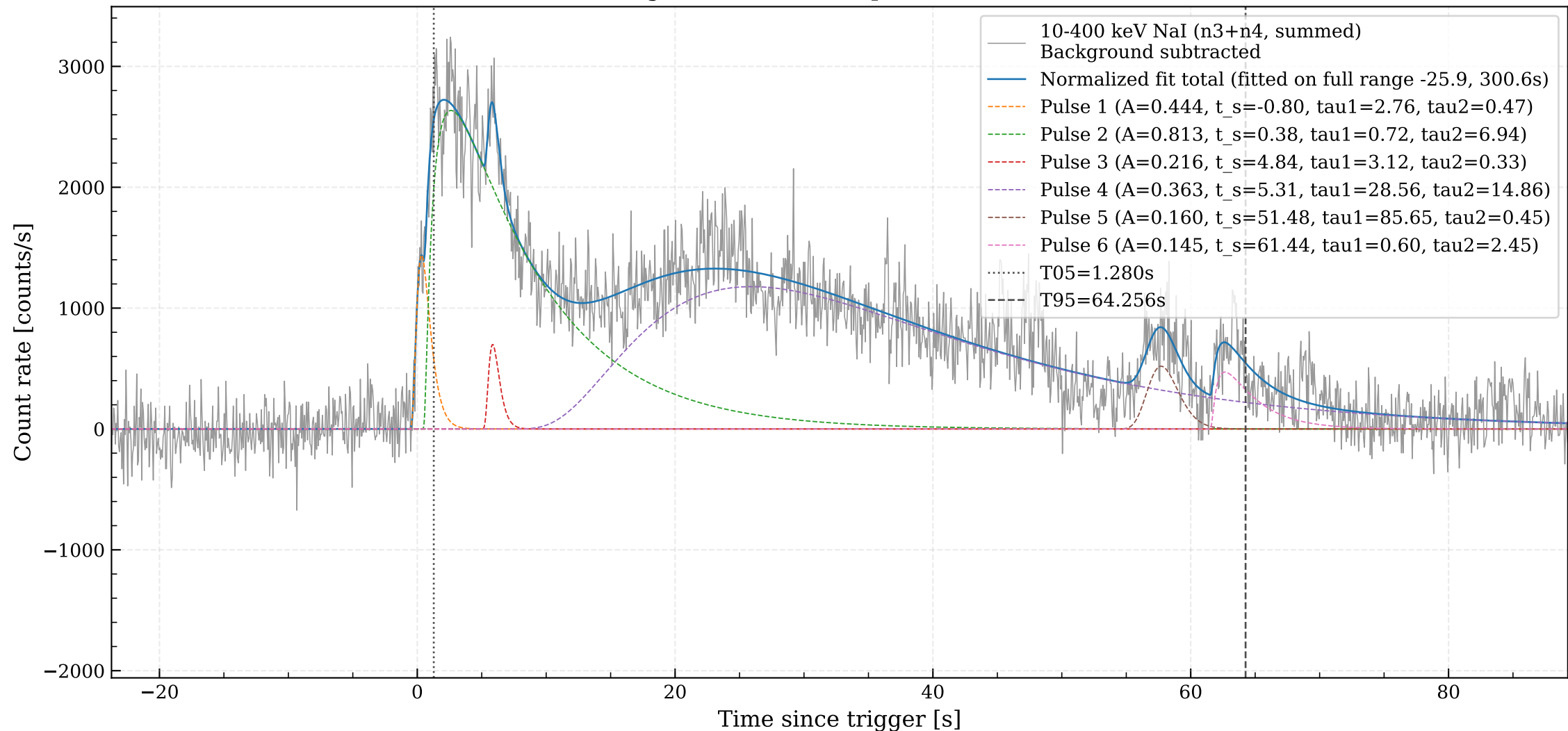
GRB080916C: full-range normalized fit (plot bounded to T05-25s, T95+25s)
