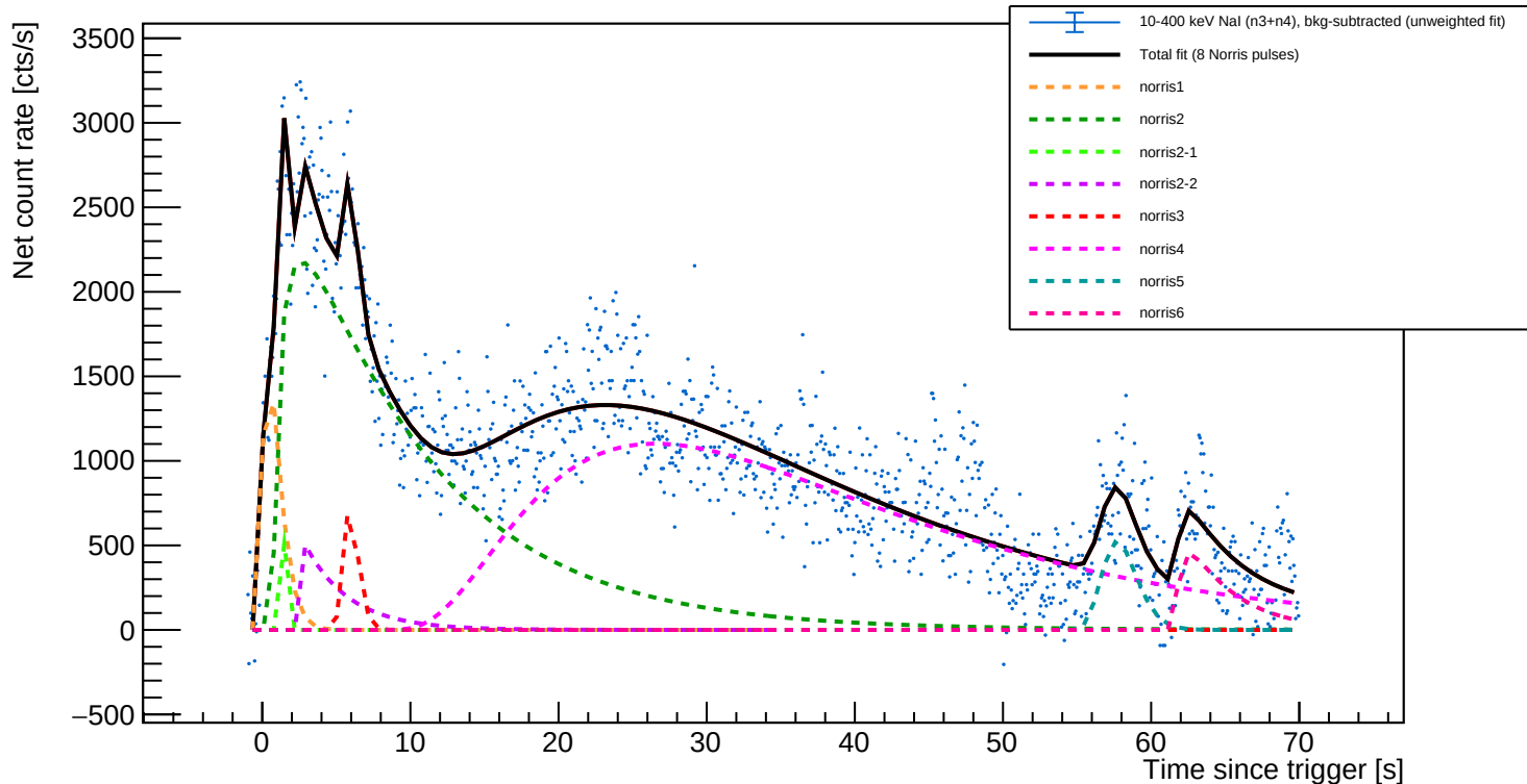
GRB080916C 10-400 keV NaI (n3+n4), background-subtracted
