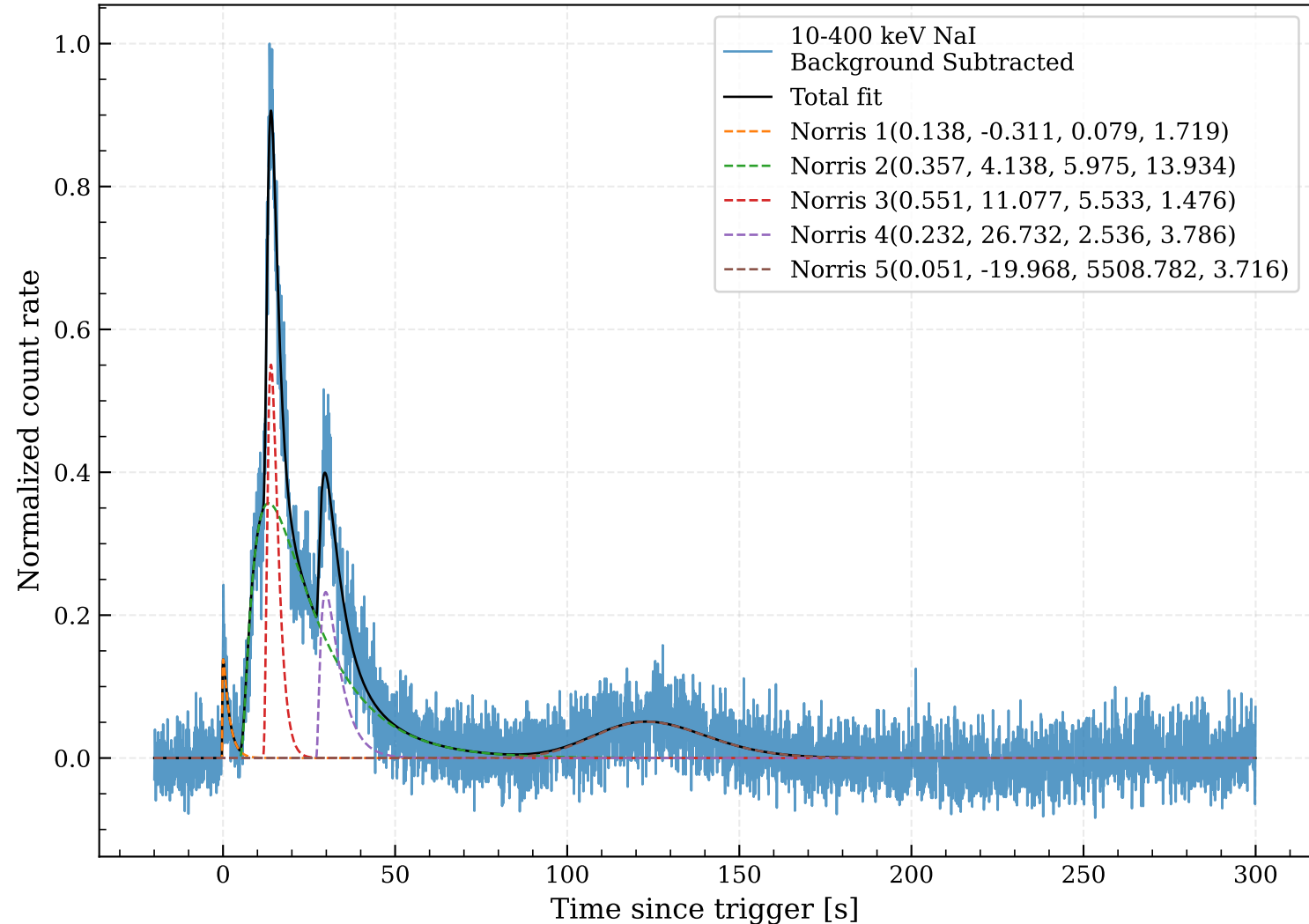
GRB140206B SIMPLE window-sensitivity check: wide_-20_300 [-20, 300] s
