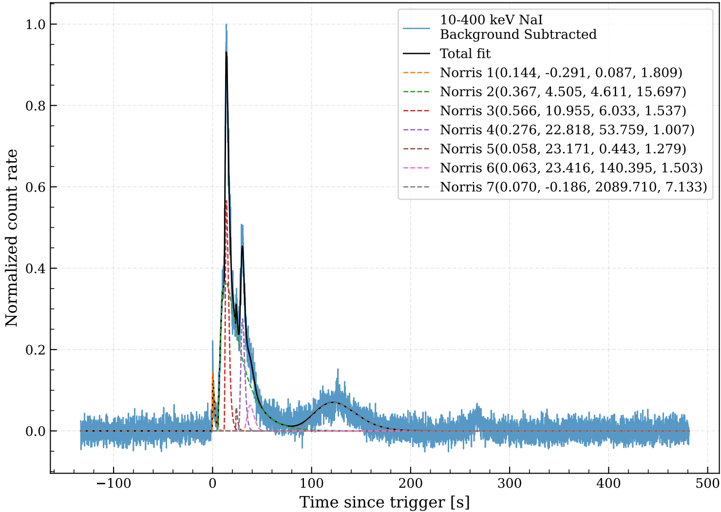
GRB140206B COMPLEX window-sensitivity check: widest_full_range [-133.184, 481.152] s
