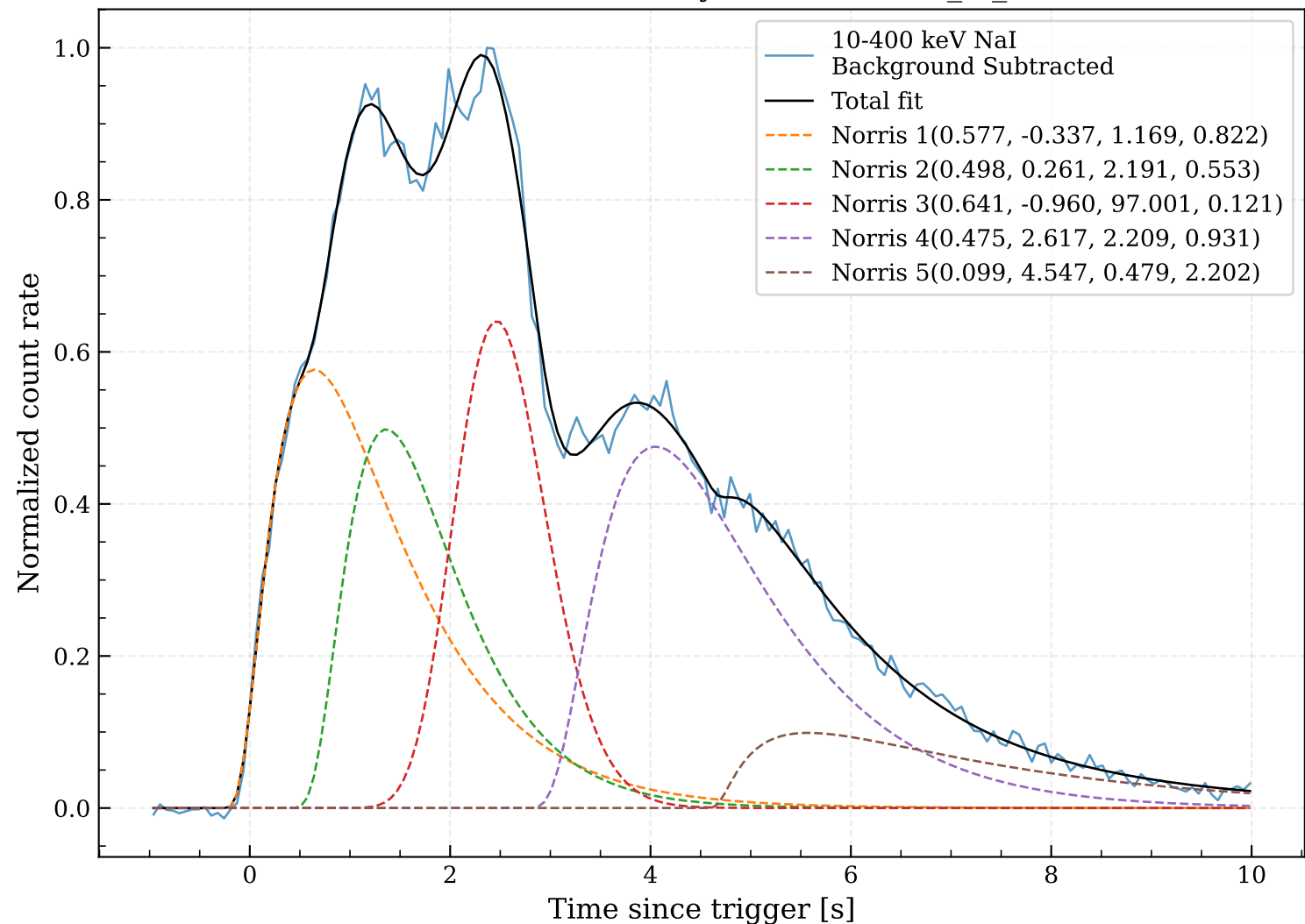
GRB231129C window-sensitivity check: narrow_1_10 [-1, 10] s
