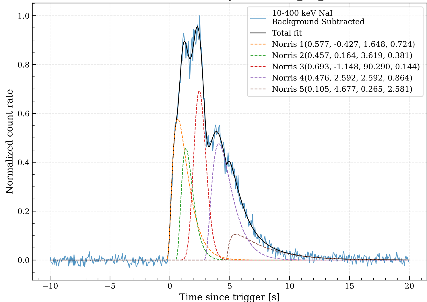
GRB231129C window-sensitivity check: wide_-10_20 [-10, 20] s
