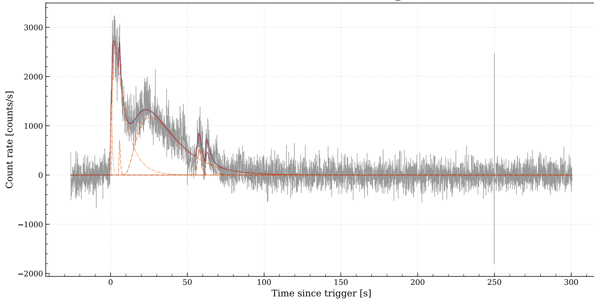
GRB080916C: normalized vs. unnormalized (x_scale) Norris fit
