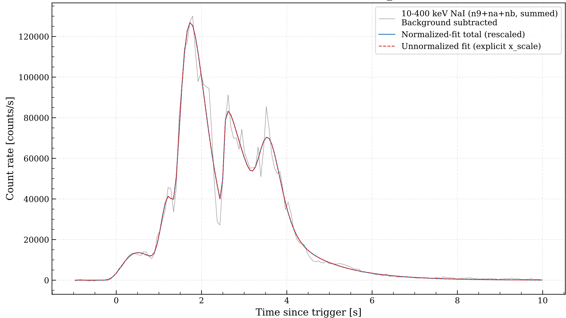
GRB131014A: normalized vs. unnormalized (x_scale) Norris fit
