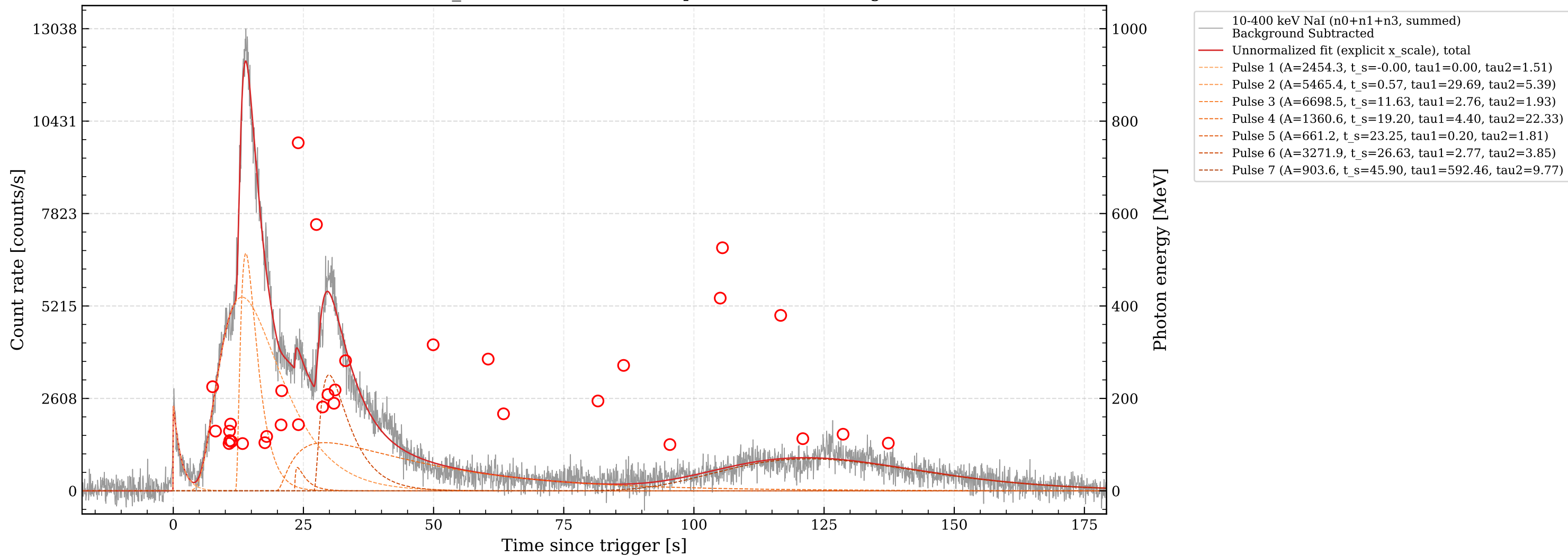
GRB140206B: unnormalized (x_scale) fit (COMPLEX, 7-pulse-2 Q0), full range -133.2-481.2s
