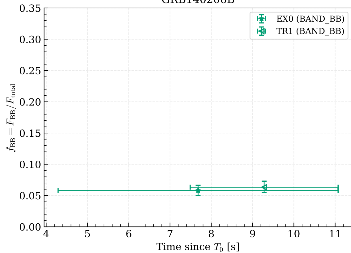
GRB140206B
