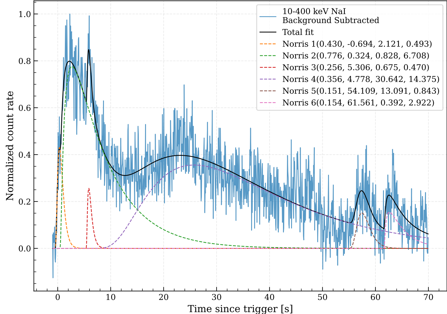
GRB080916C SIX-pulse window-sensitivity check: narrow_-1_70 [-1, 70] s
