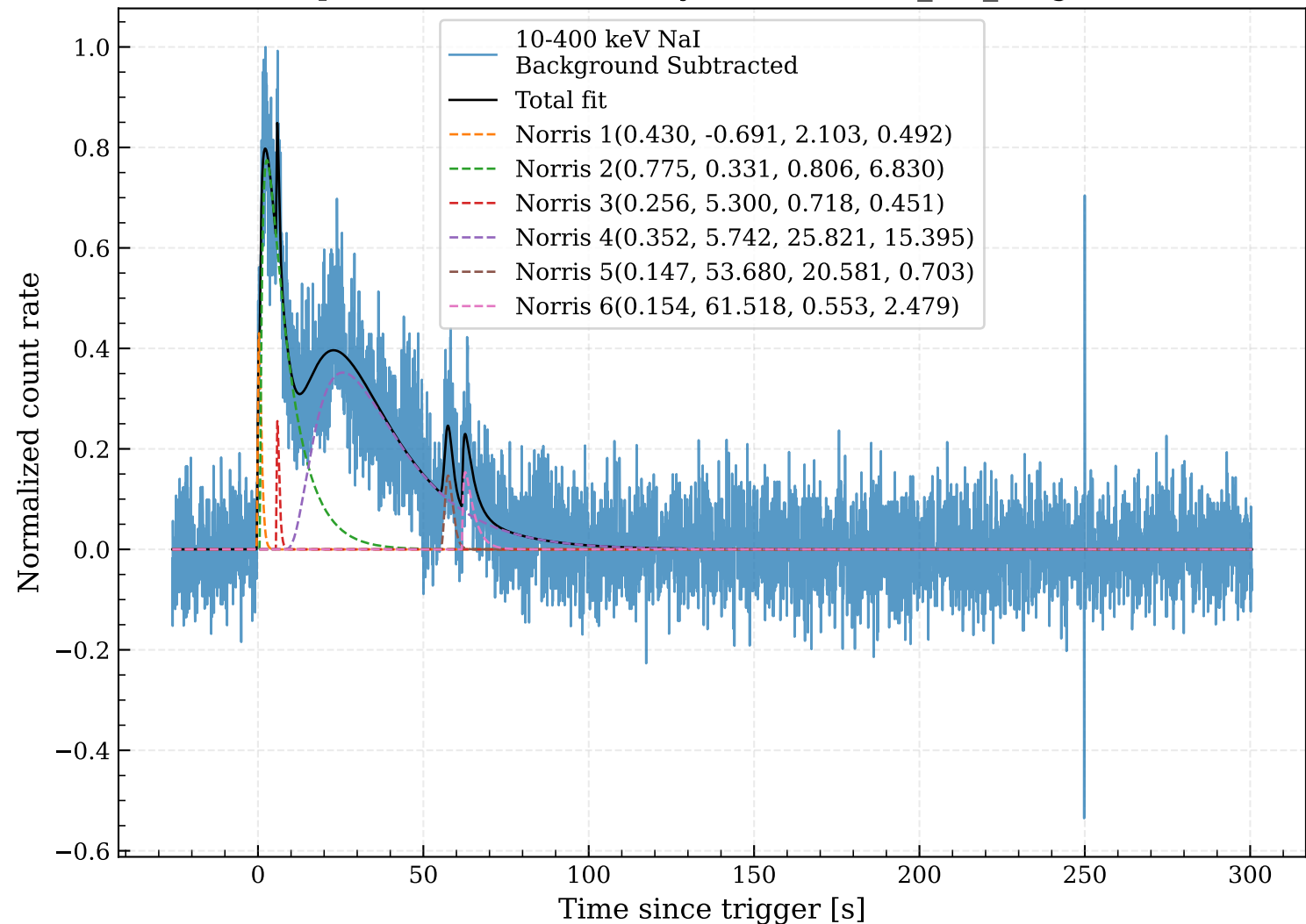
GRB080916C SIX-pulse window-sensitivity check: widest_full_range [-25.92, 300.608] s
