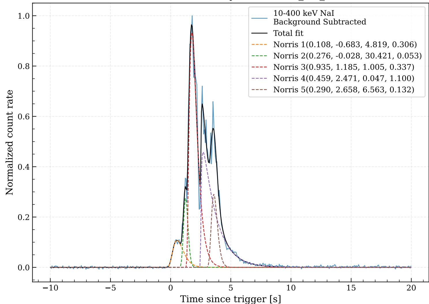
GRB131014A window-sensitivity check: wide_-10_20 [-10, 20] s
