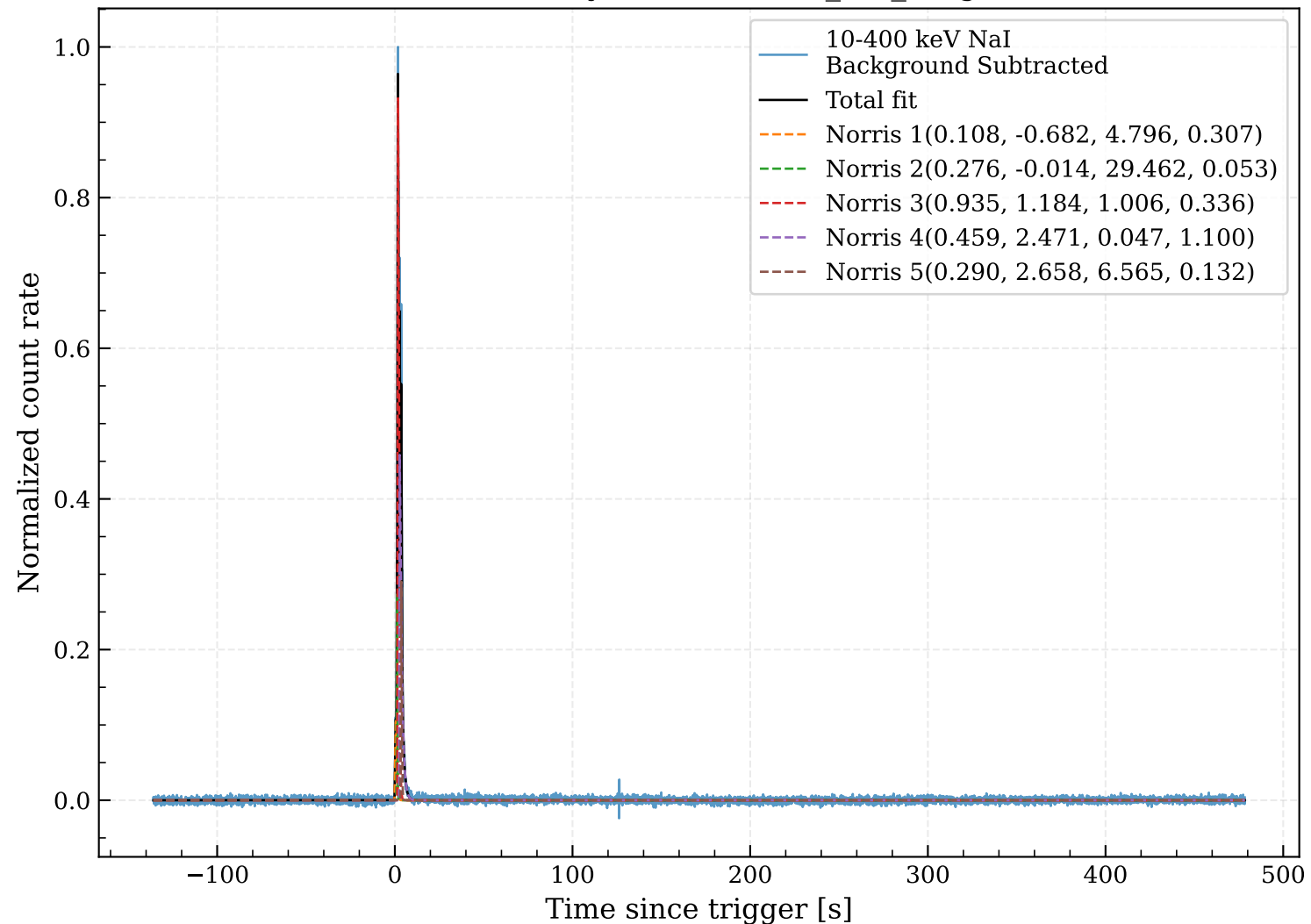
GRB131014A window-sensitivity check: widest_full_range [-135.936, 478.4] s
