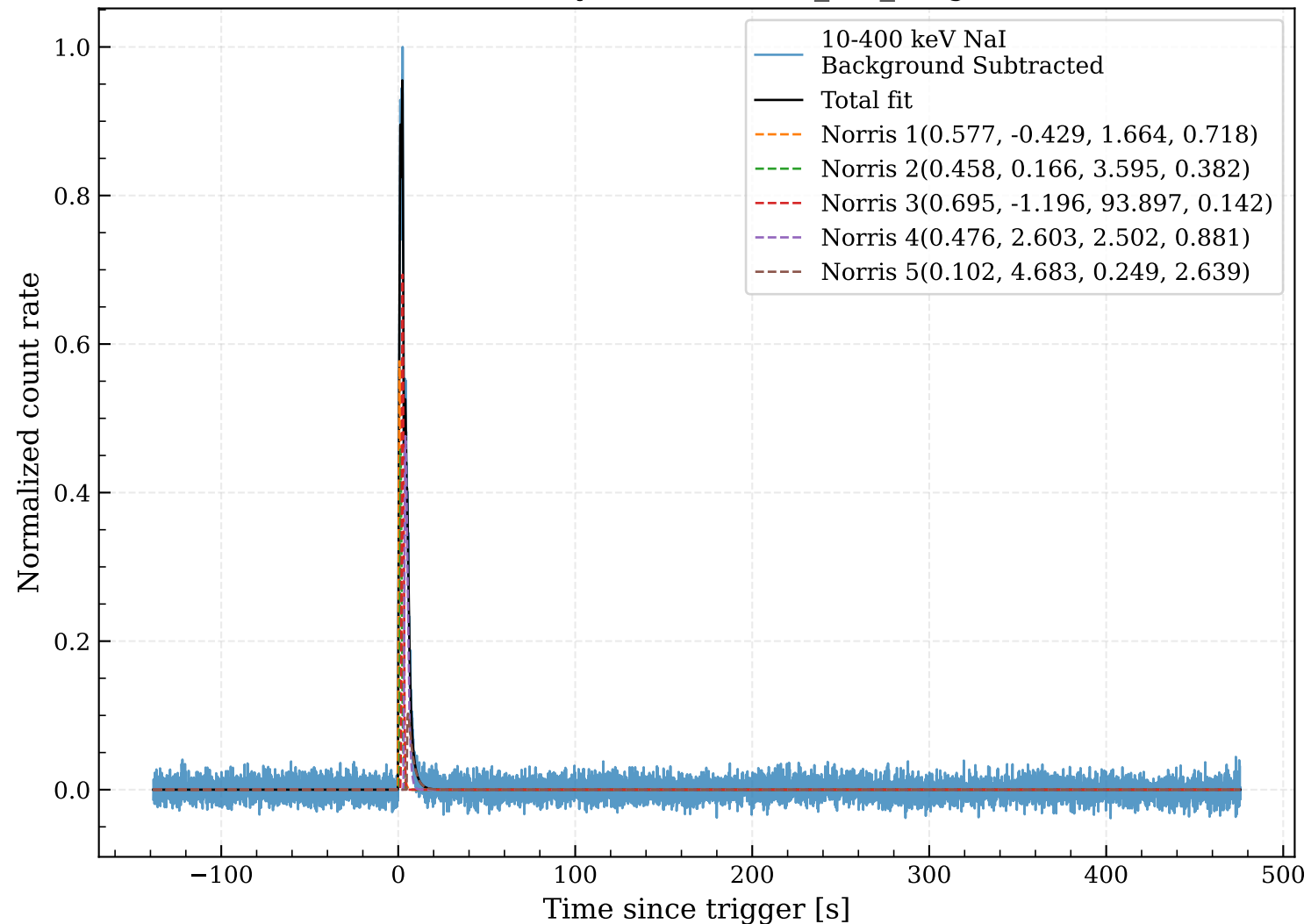
GRB231129C window-sensitivity check: widest_full_range [-138.496, 475.84] s
